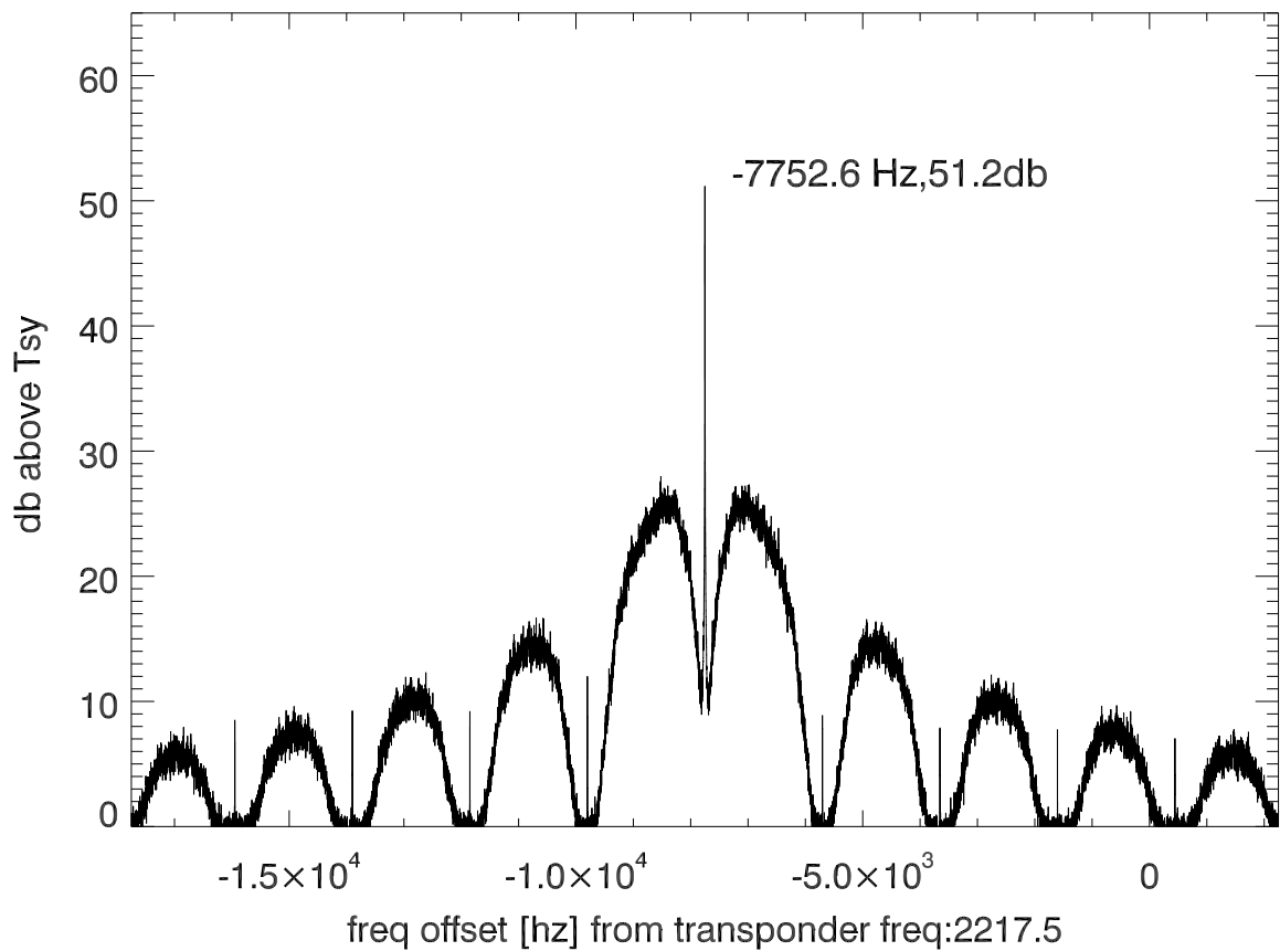
isee3 140627:192110 (UTC) spectra after doppler correction. PoIB
