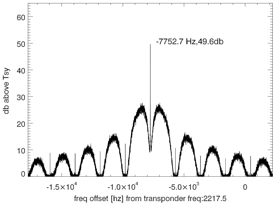
isee3 140627:191814 (UTC) spectra after doppler correction. PoIB
