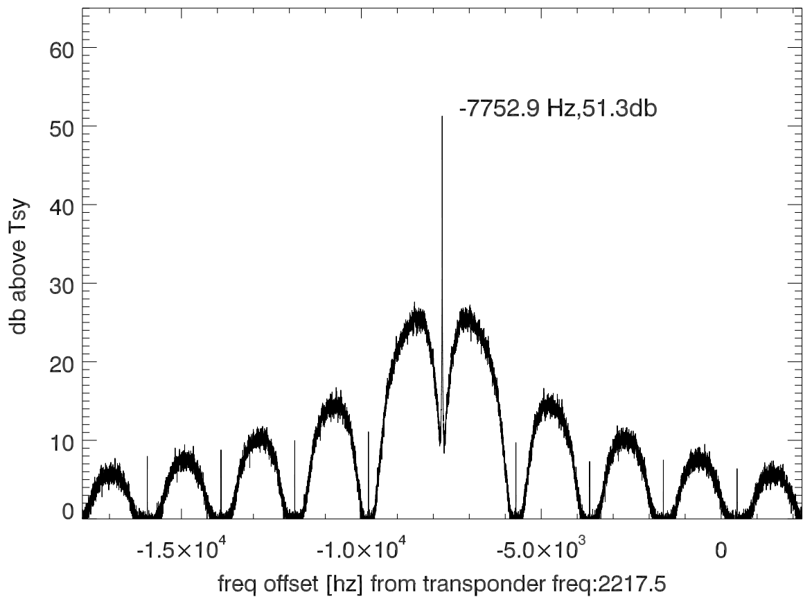
isee3 140627:191525 (UTC) spectra after doppler correction. PoIB
