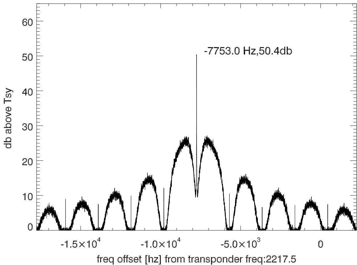
isee3 140627:191045 (UTC) spectra after doppler correction. PoIB
