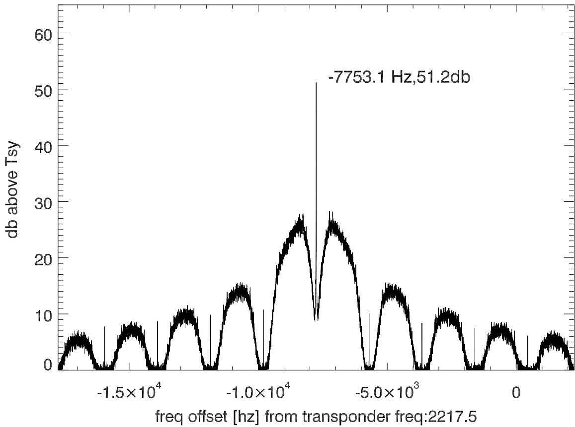
isee3 140627:190446 (UTC) spectra after doppler correction. PoIB
