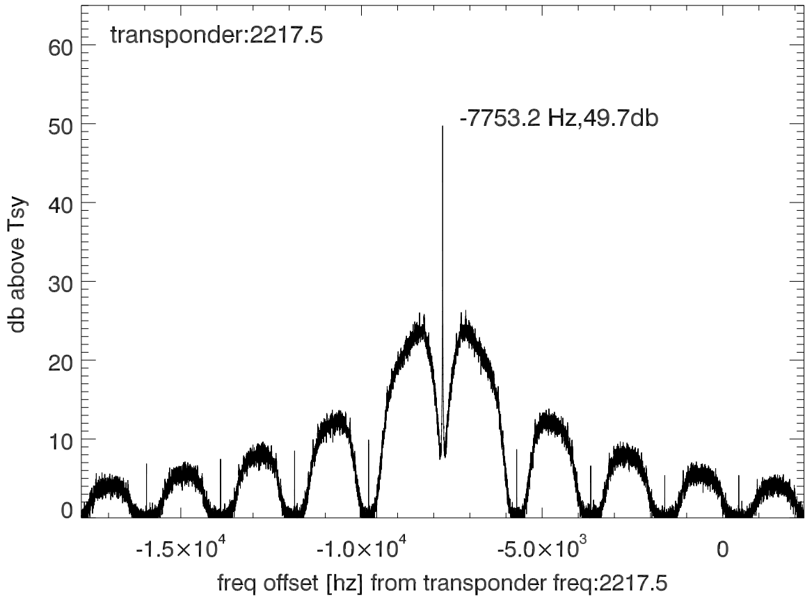
isee3 140627:190446 (UTC) spectra after doppler correction. PoIA
