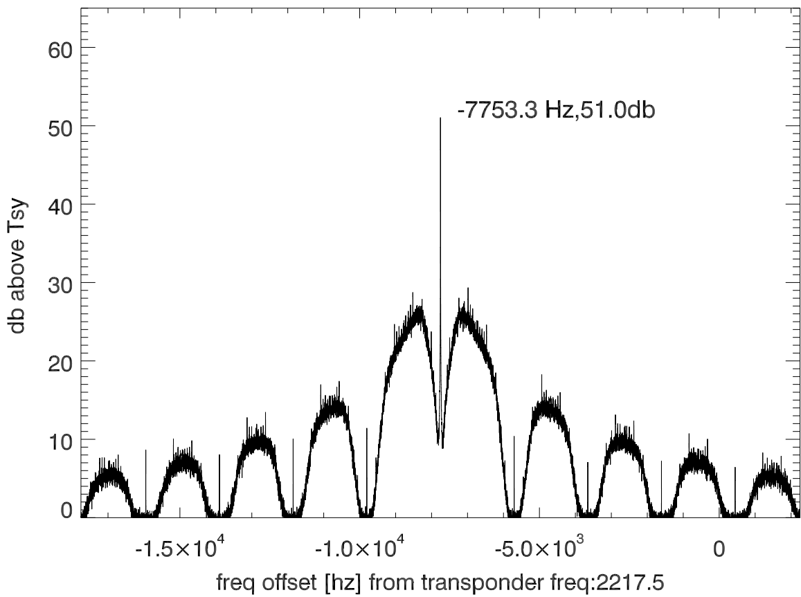
isee3 140627:185809 (UTC) spectra after doppler correction. PoIB
