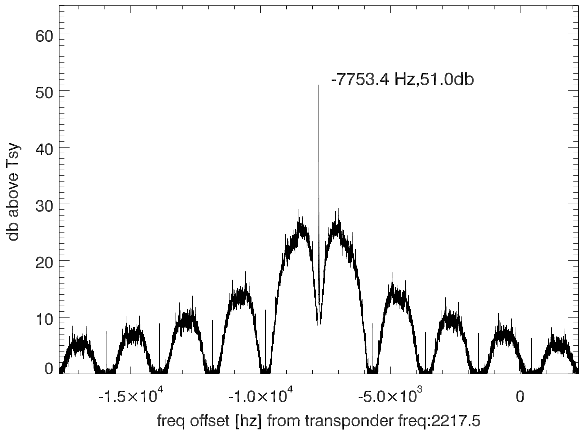
isee3 140627:185329 (UTC) spectra after doppler correction. PoIB
