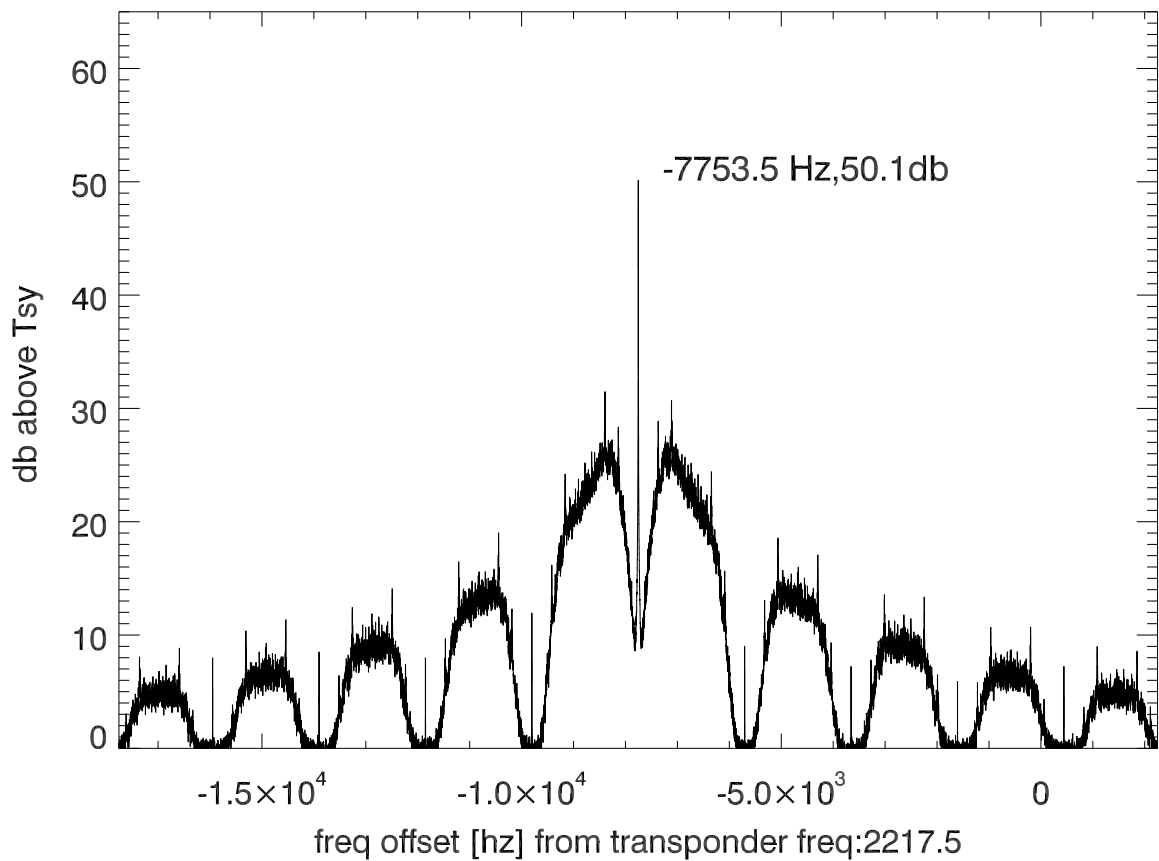
isee3 140627:185027 (UTC) spectra after doppler correction. PoIB
