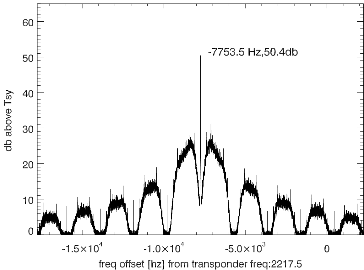
isee3 140627:184809 (UTC) spectra after doppler correction. PoIB
