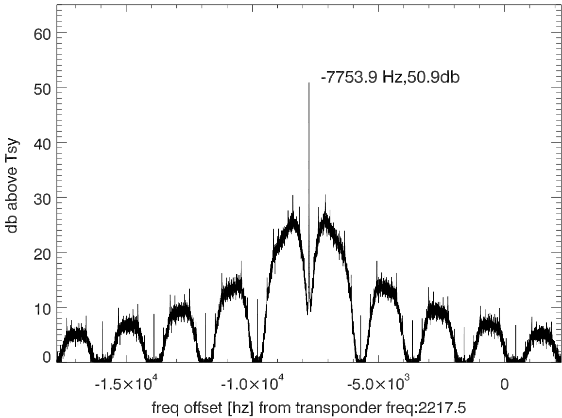
isee3 140627:182955 (UTC) spectra after doppler correction. PoIB
