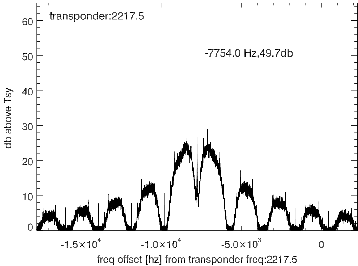
isee3 140627:182444 (UTC) spectra after doppler correction. PoIA
