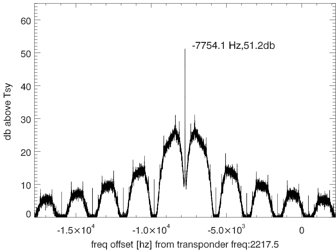
isee3 140627:182444 (UTC) spectra after doppler correction. PoIB
