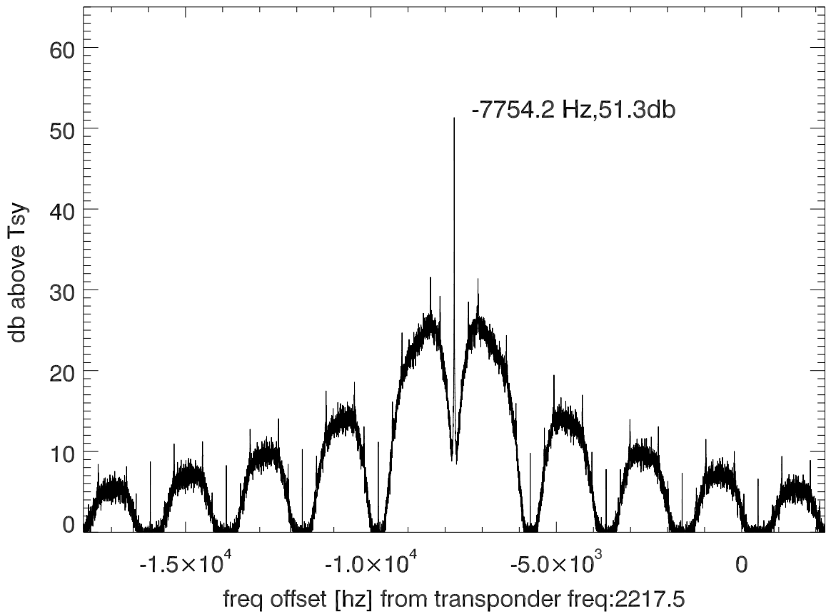
isee3 140627:182204 (UTC) spectra after doppler correction. PoIB
