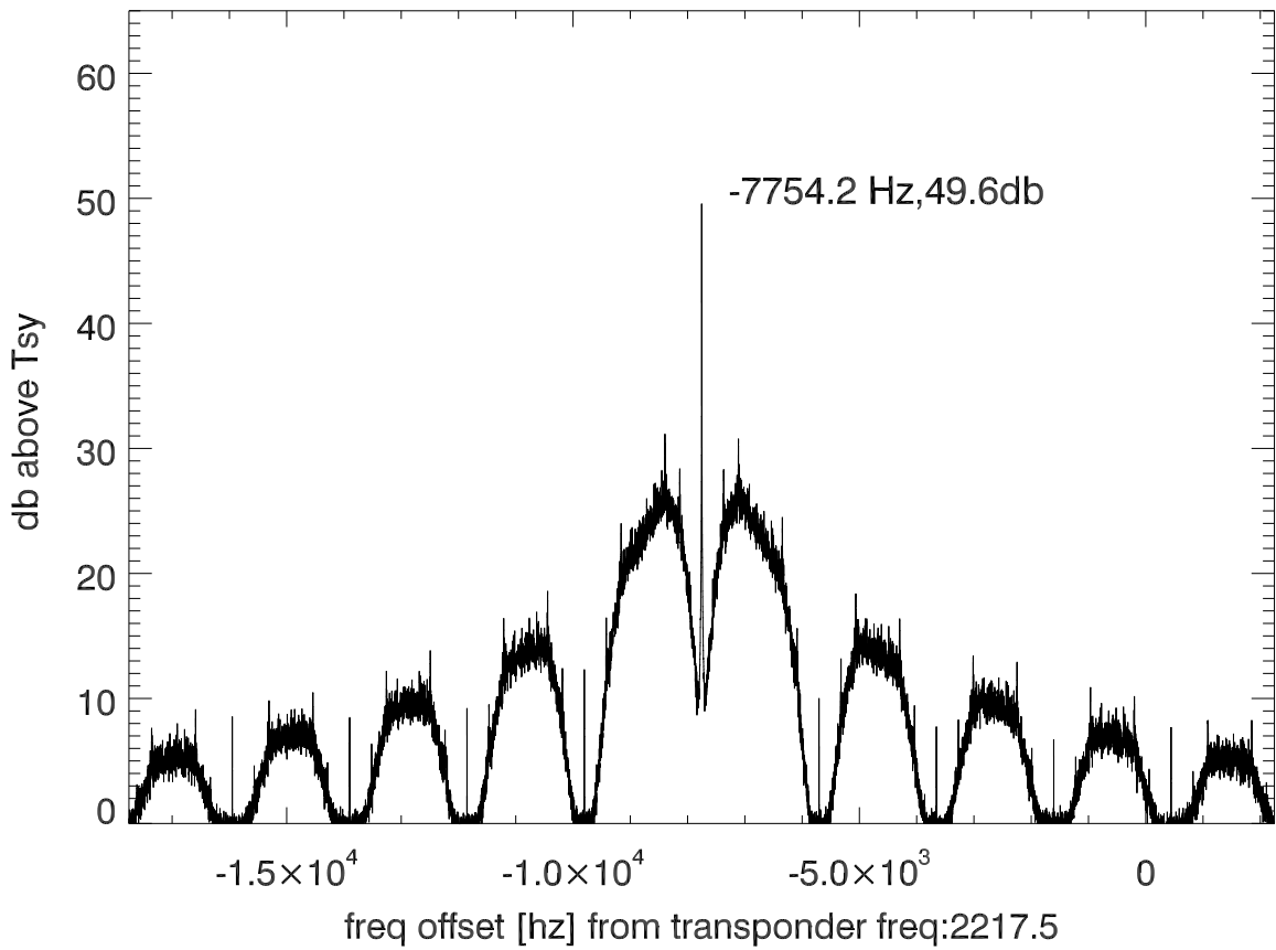
isee3 140627:181940 (UTC) spectra after doppler correction. PoIB
