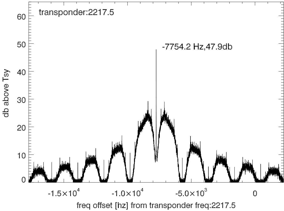
isee3 140627:181940 (UTC) spectra after doppler correction. PoIA
