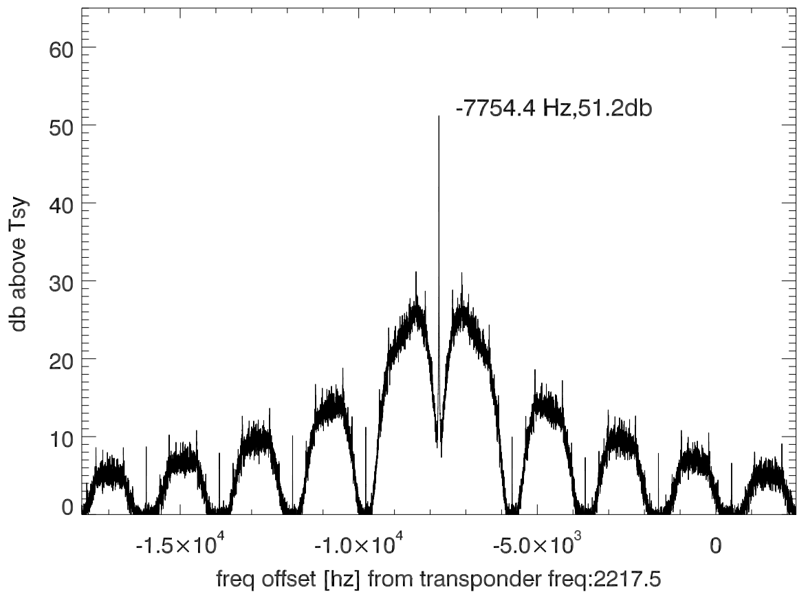
isee3 140627:181630 (UTC) spectra after doppler correction. PoIB
