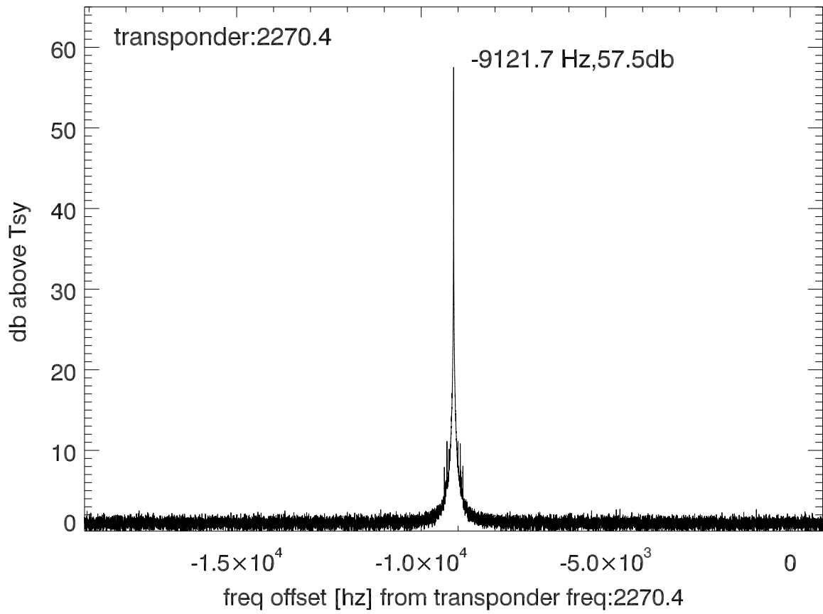
isee3 140625:181847 (UTC) spectra after doppler correction. PolA
