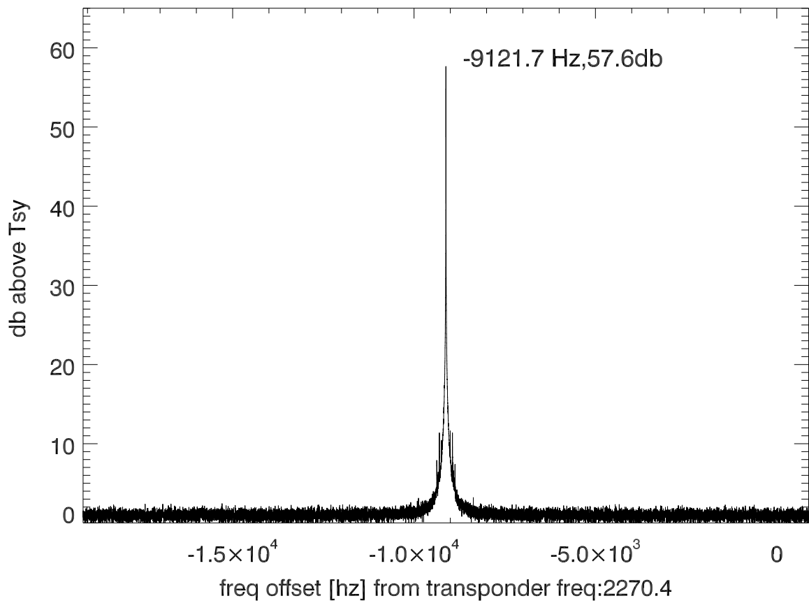
isee3 140625:181847 (UTC) spectra after doppler correction. PolB
