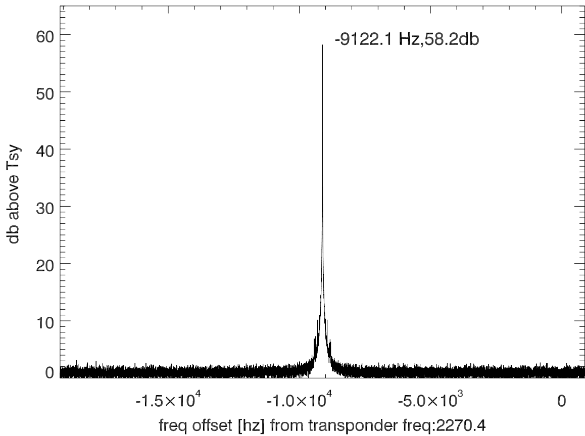
isee3 140625:181241 (UTC) spectra after doppler correction. PolB
