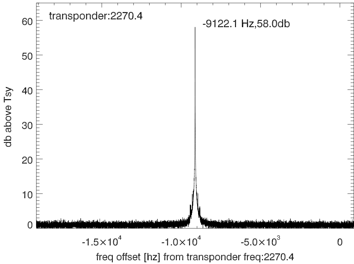
isee3 140625:181241 (UTC) spectra after doppler correction. PolA
