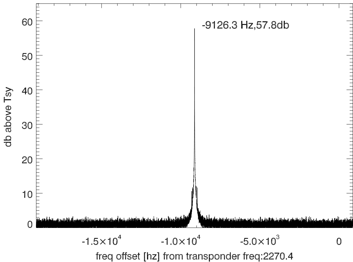
isee3 140625:180254 (UTC) spectra after doppler correction. PolB
