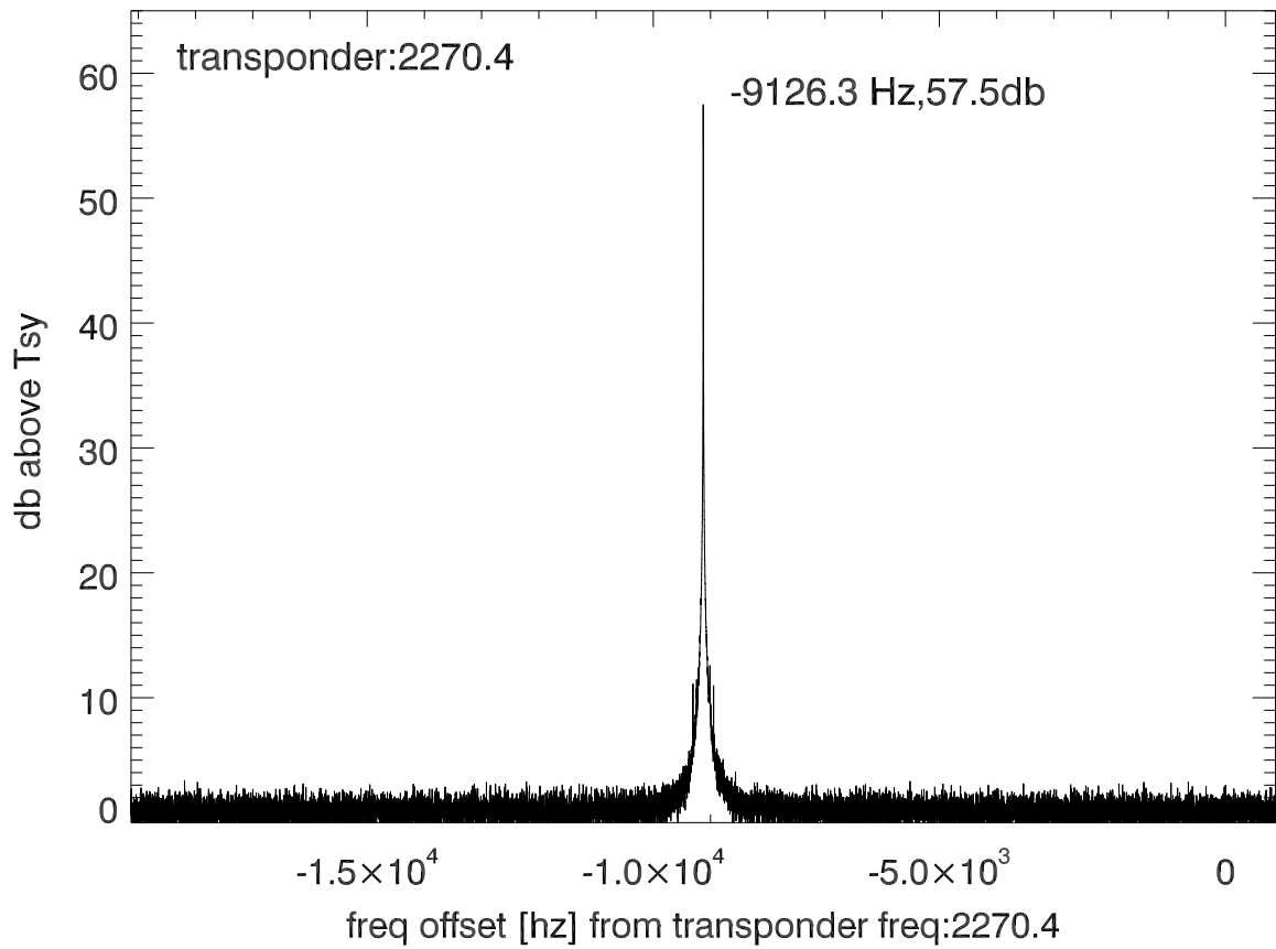
isee3 140625:180254 (UTC) spectra after doppler correction. PolA
