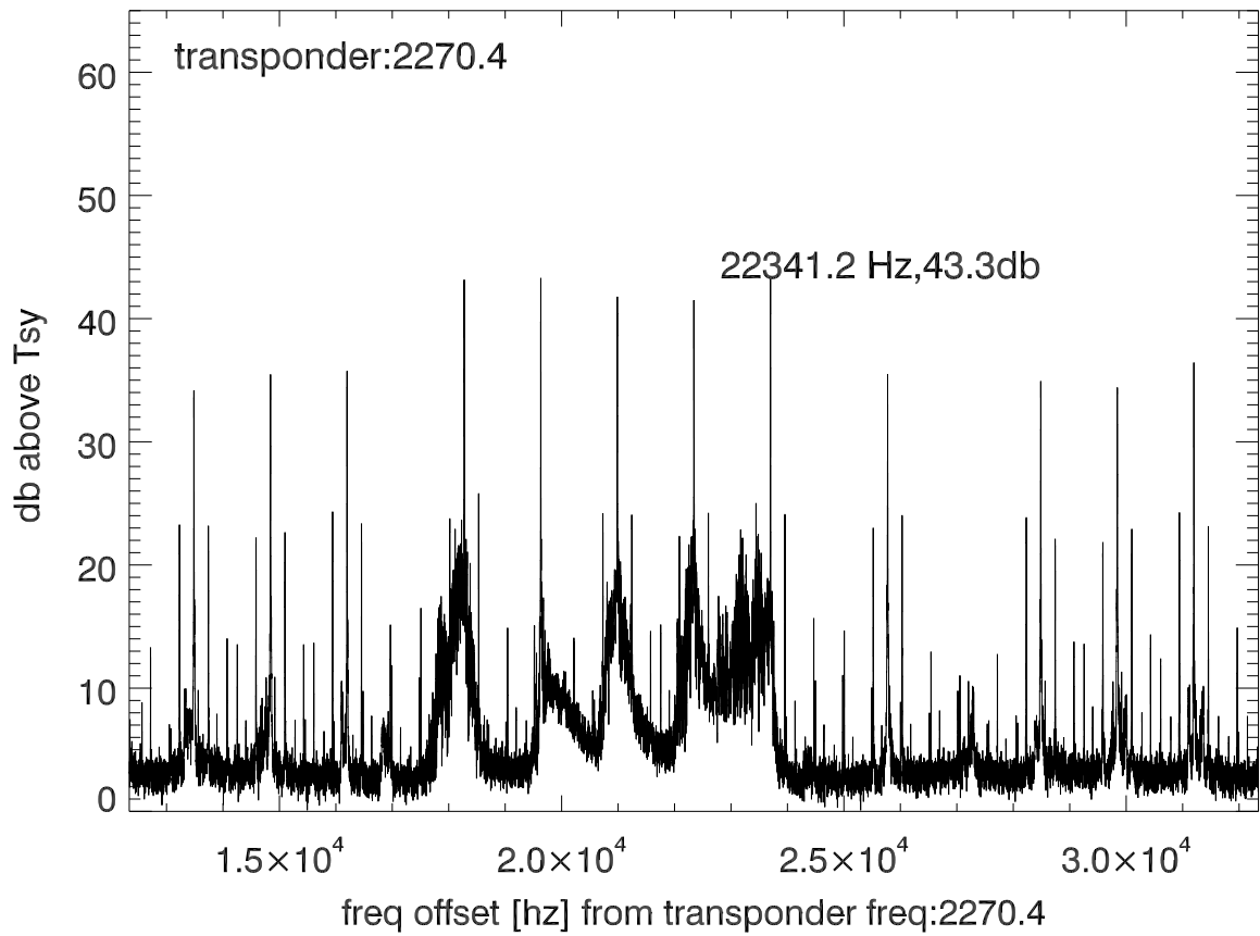
isee3 140625:180002 (UTC) spectra after doppler correction. PolA
