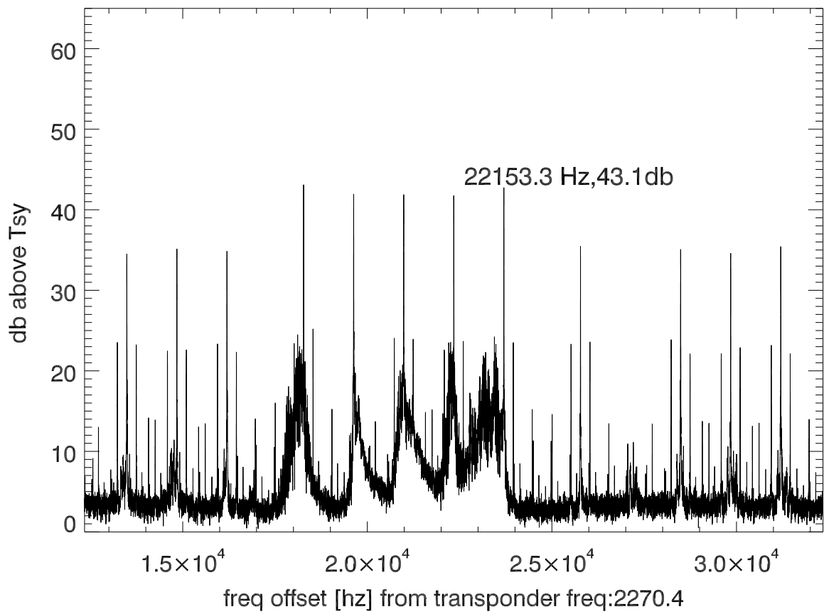
isee3 140625:180002 (UTC) spectra after doppler correction. PolB
