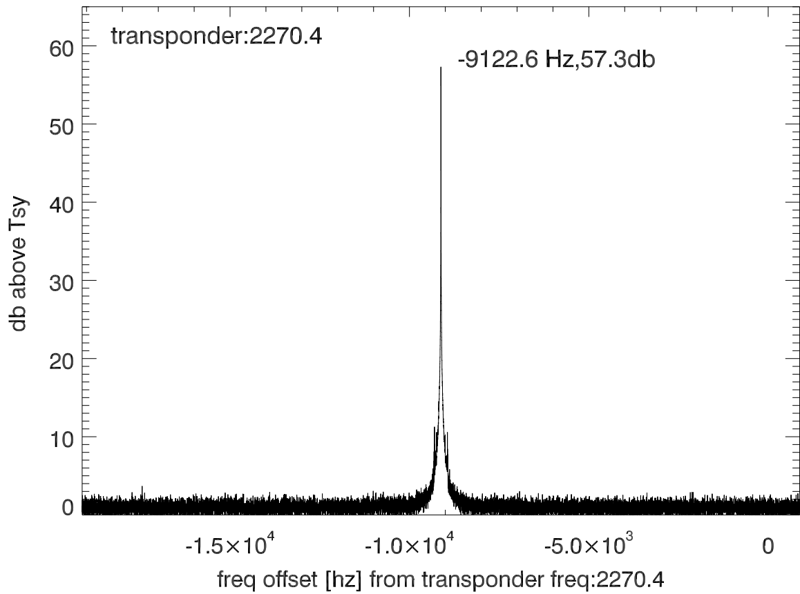
isee3 140625:175646 (UTC) spectra after doppler correction. PolA
