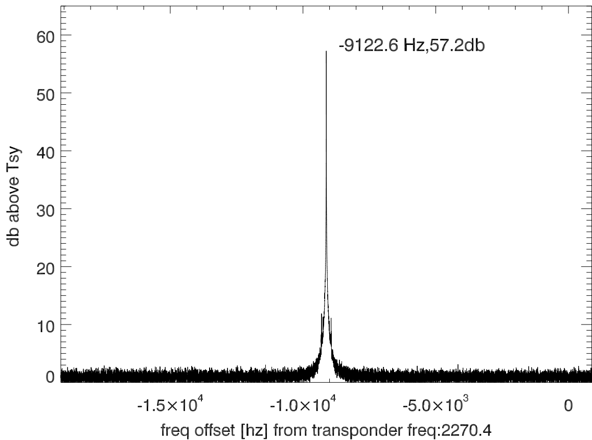
isee3 140625:175646 (UTC) spectra after doppler correction. PolB
