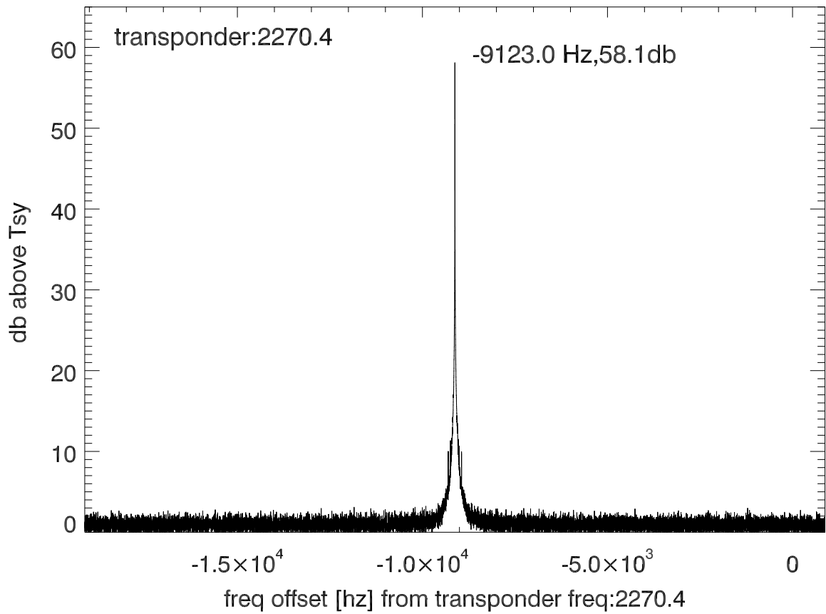
isee3 140625:175349 (UTC) spectra after doppler correction. PolA
