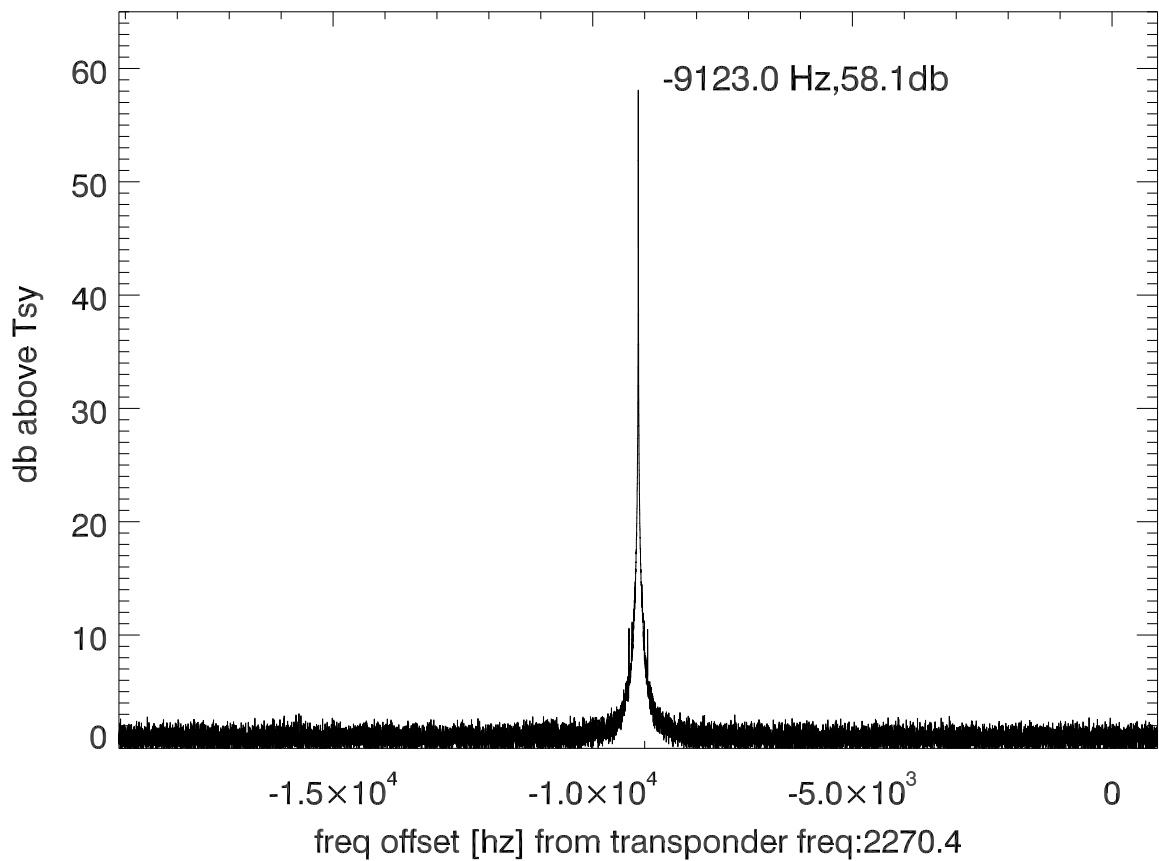
isee3 140625:175349 (UTC) spectra after doppler correction. PolB
