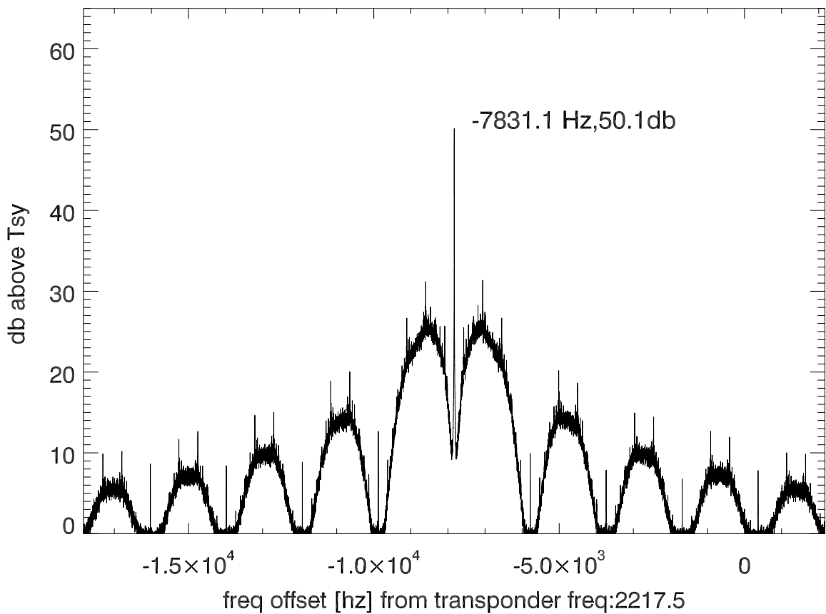
isee3 140625:180730 (UTC) spectra after doppler correction. PoIB
