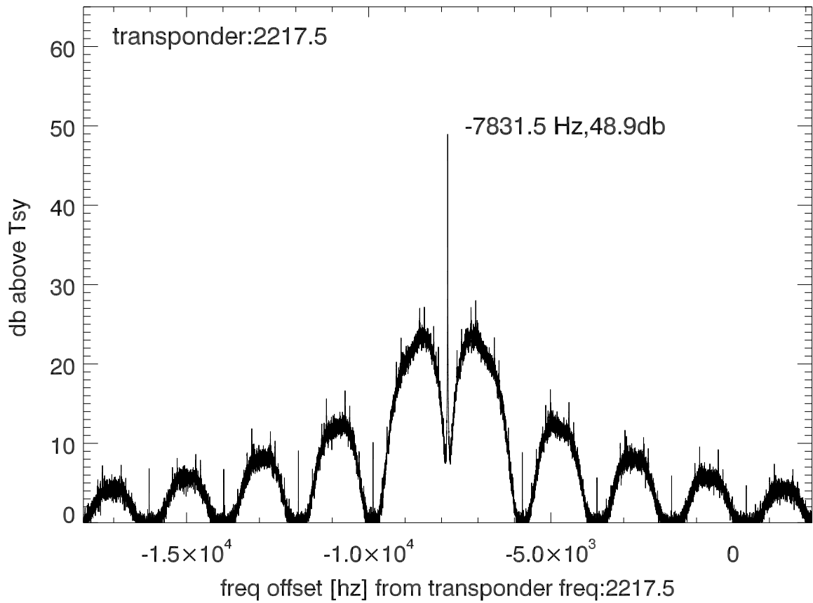
isee3 140625:175349 (UTC) spectra after doppler correction. PoIA
