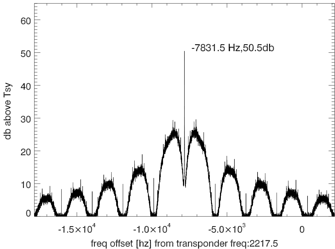
isee3 140625:175349 (UTC) spectra after doppler correction. PoIB
