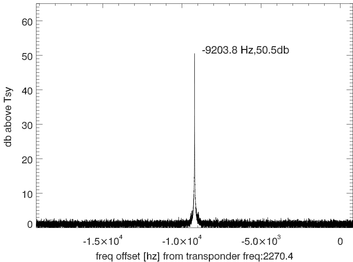
isee3 140624:200902 (UTC) spectra after doppler correction. PolB
