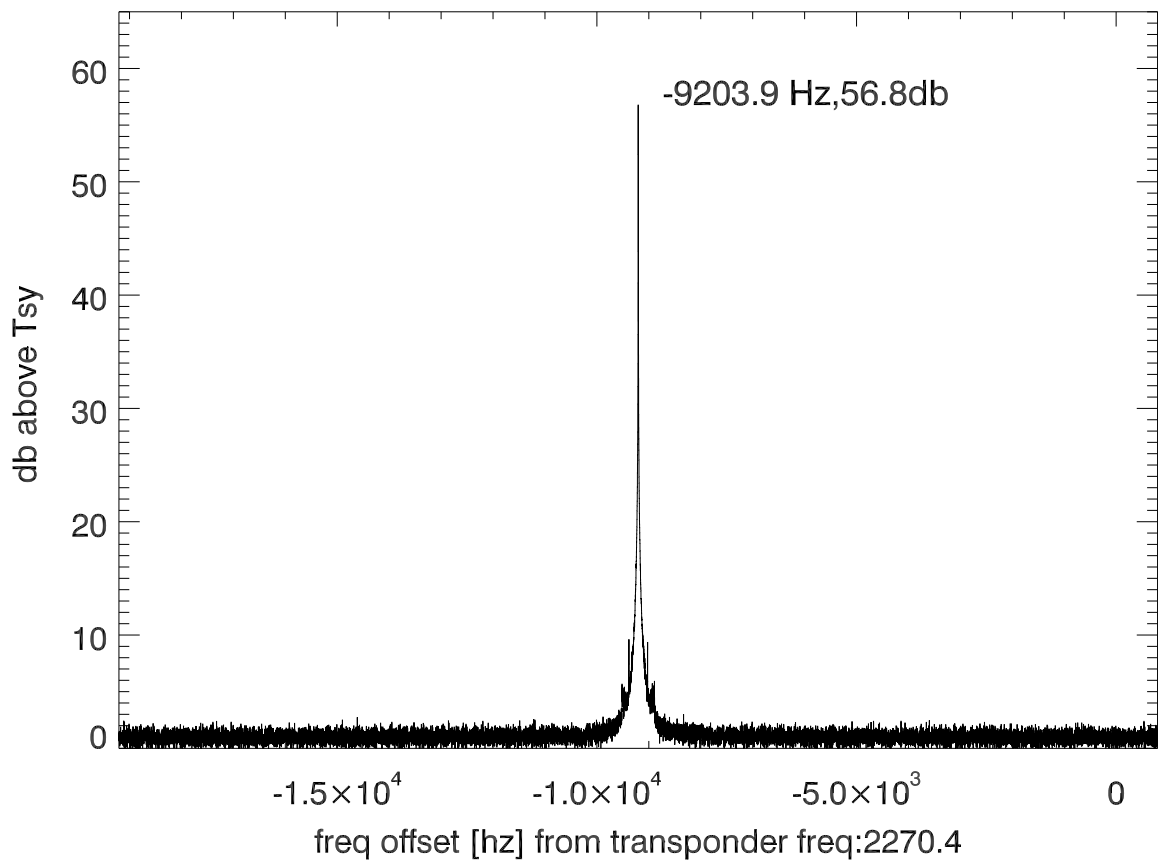
isee3 140624:200519 (UTC) spectra after doppler correction. PolB
