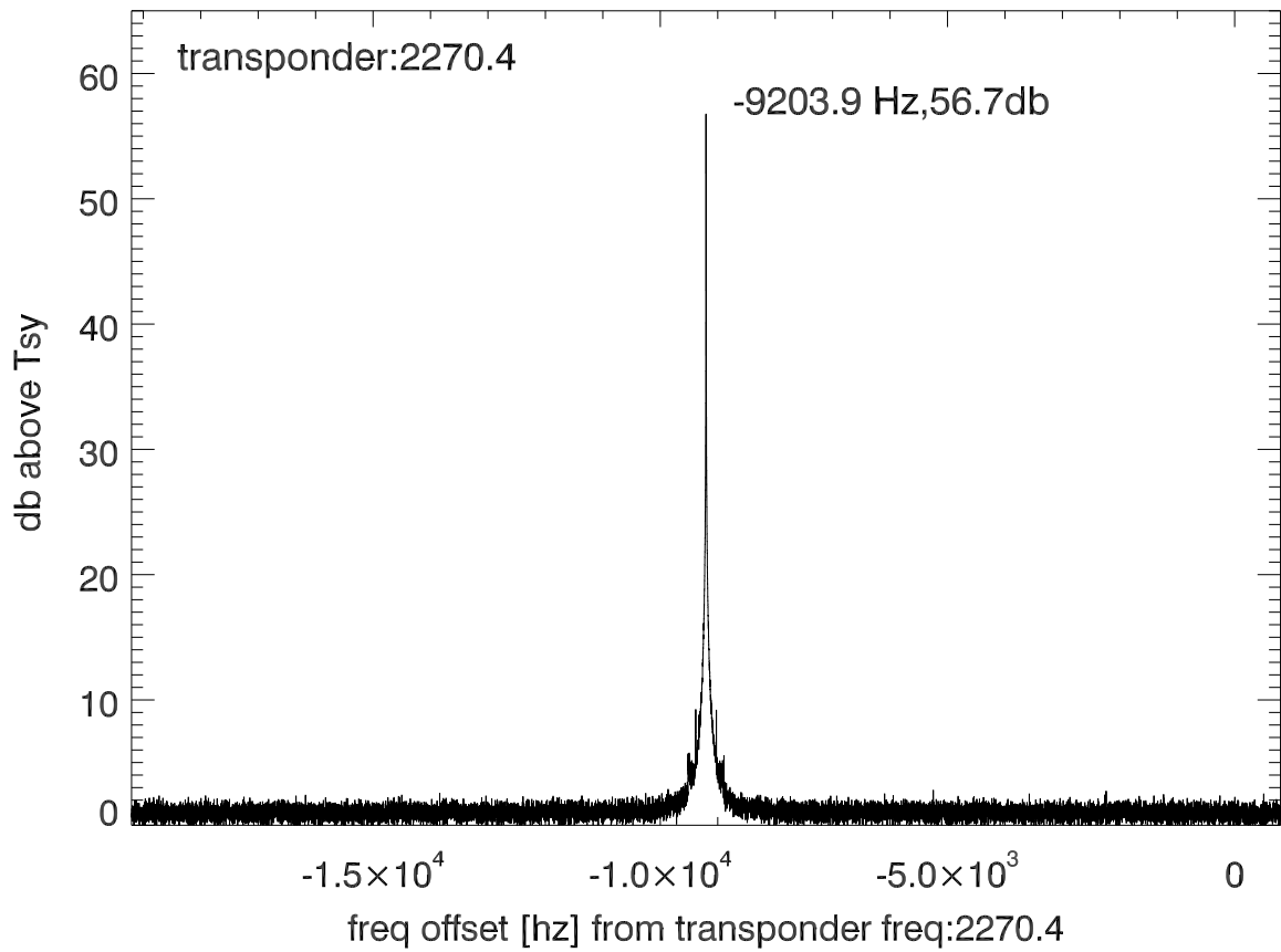
isee3 140624:200519 (UTC) spectra after doppler correction. PolA
