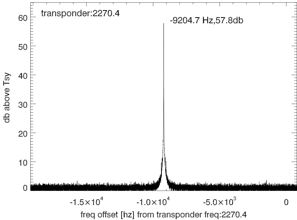
isee3 140624:195135 (UTC) spectra after doppler correction. PolA
