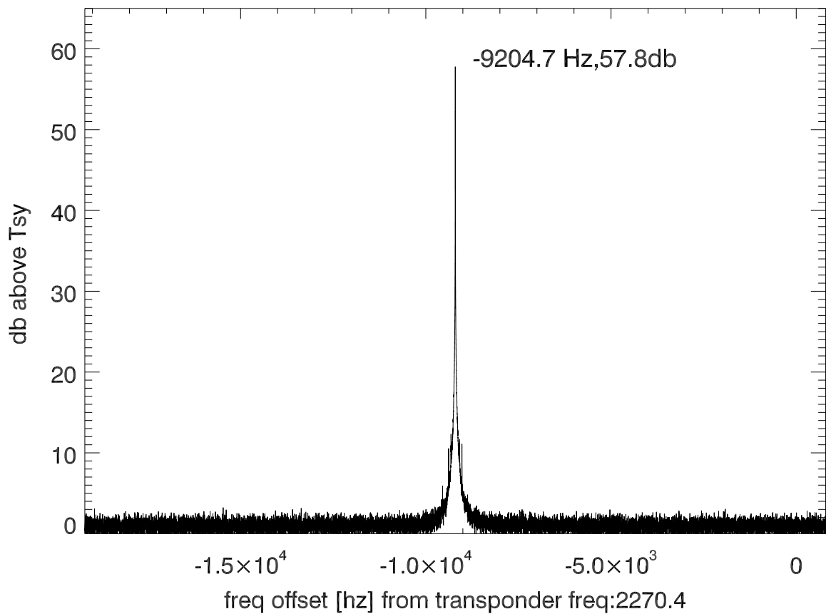
isee3 140624:195135 (UTC) spectra after doppler correction. PolB
