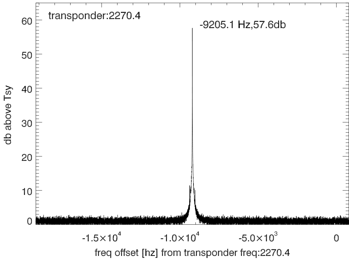
isee3 140624:194457 (UTC) spectra after doppler correction. PolA
