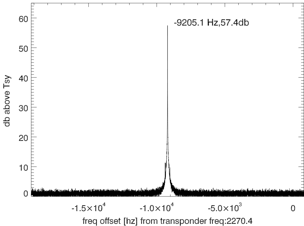
isee3 140624:194457 (UTC) spectra after doppler correction. PolB
