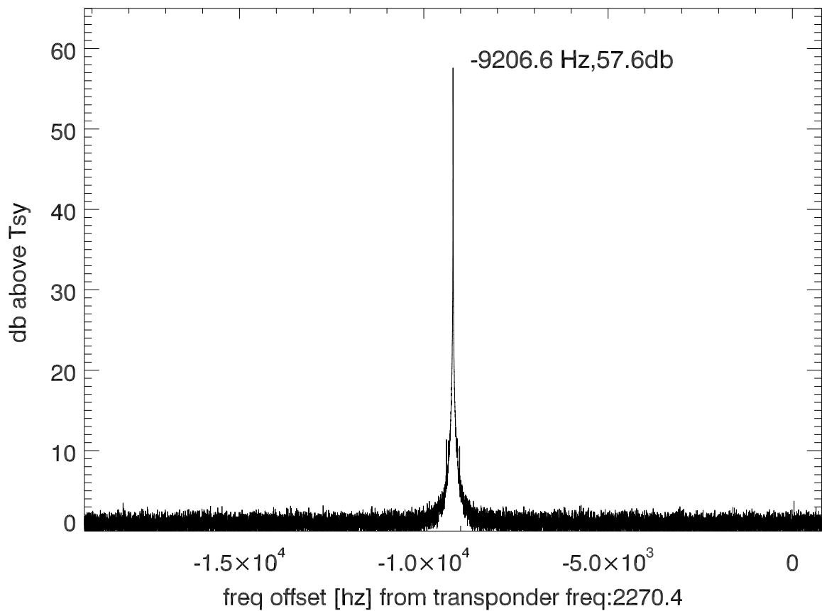
isee3 140624:193239 (UTC) spectra after doppler correction. PolB
