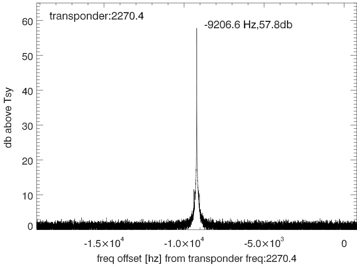
isee3 140624:193239 (UTC) spectra after doppler correction. PolA
