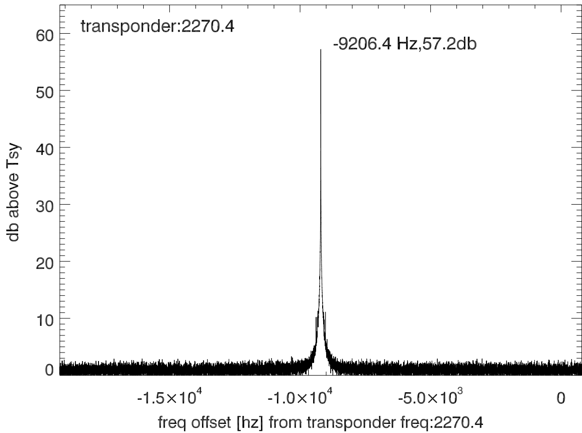
isee3 140624:192537 (UTC) spectra after doppler correction. PolA
