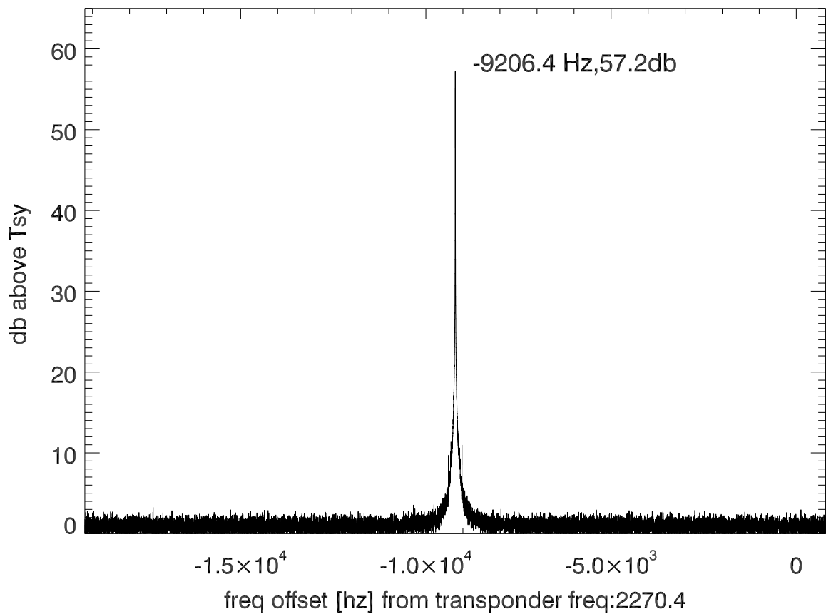
isee3 140624:192537 (UTC) spectra after doppler correction. PolB
