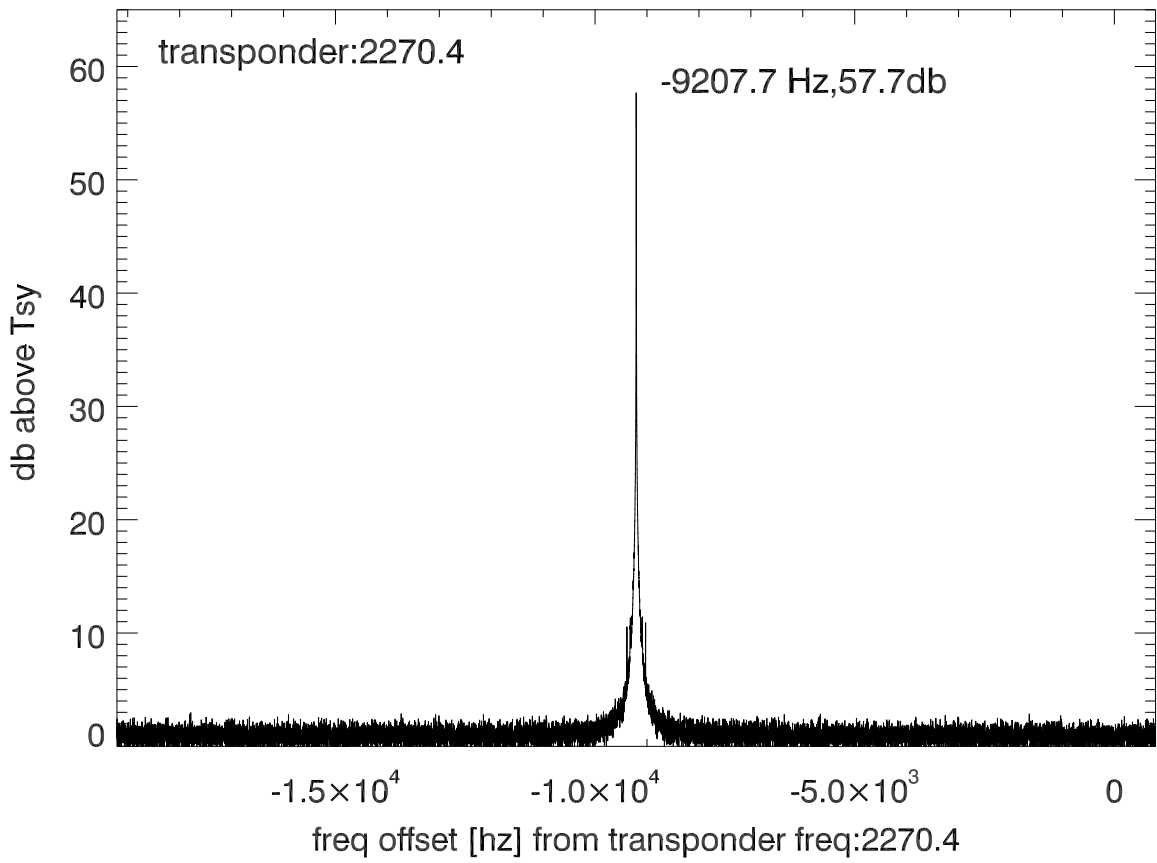
isee3 140624:190905 (UTC) spectra after doppler correction. PolA
