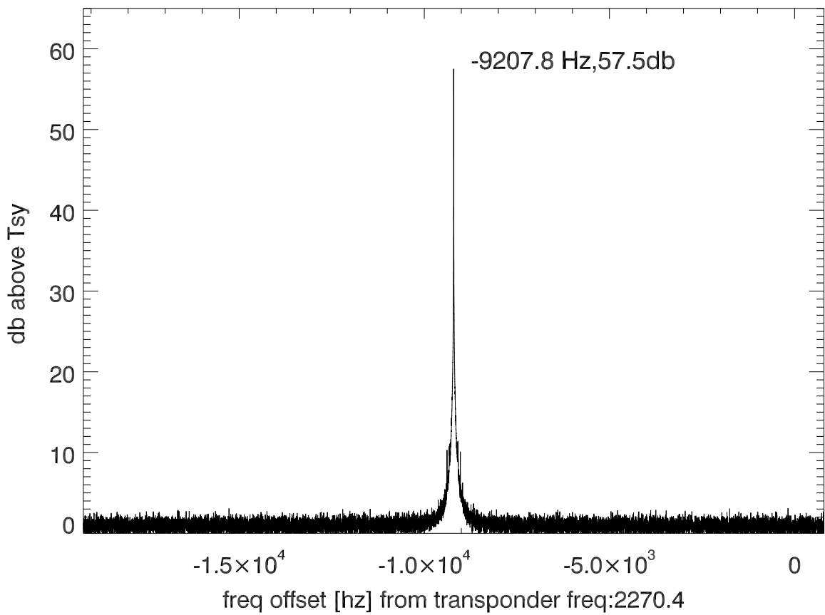
isee3 140624:190905 (UTC) spectra after doppler correction. PolB
