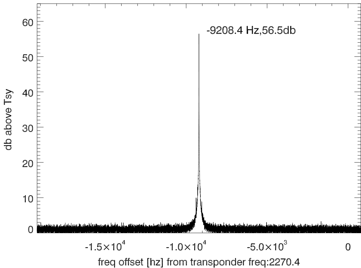
isee3 140624:190527 (UTC) spectra after doppler correction. PolB
