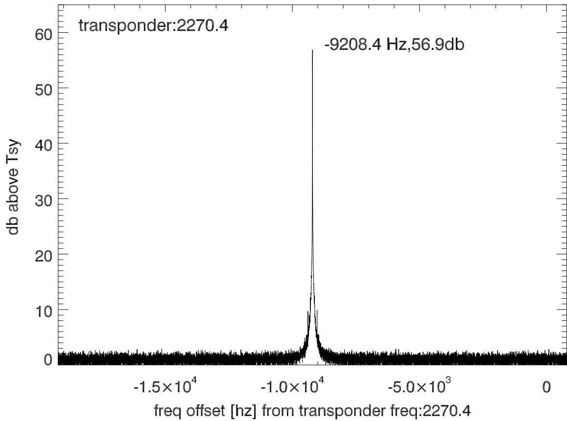
isee3 140624:190527 (UTC) spectra after doppler correction. PolA
