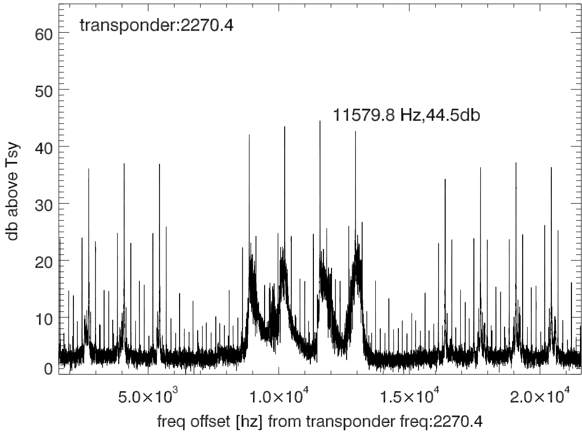
isee3 140624:185749 (UTC) spectra after doppler correction. PolA
