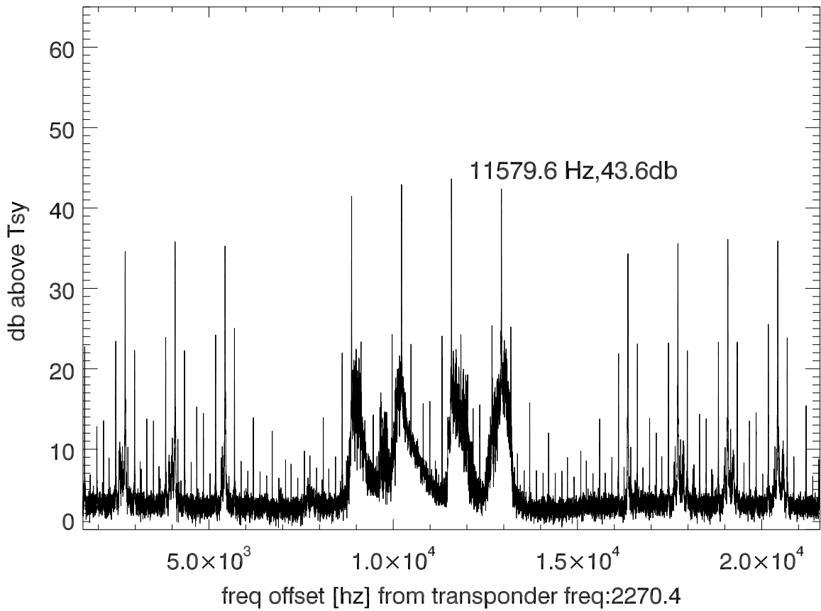
isee3 140624:185749 (UTC) spectra after doppler correction. PolB
