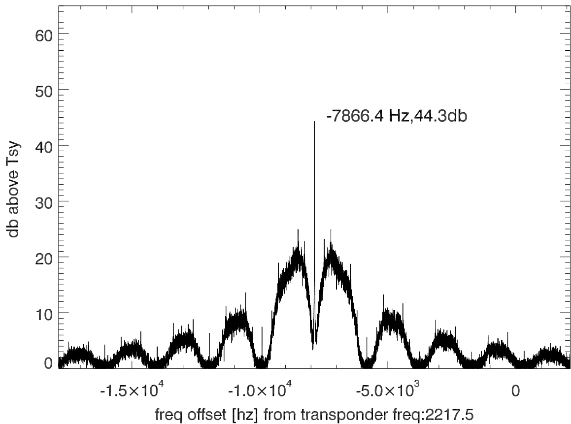
isee3 140624:200902 (UTC) spectra after doppler correction. PoIB
