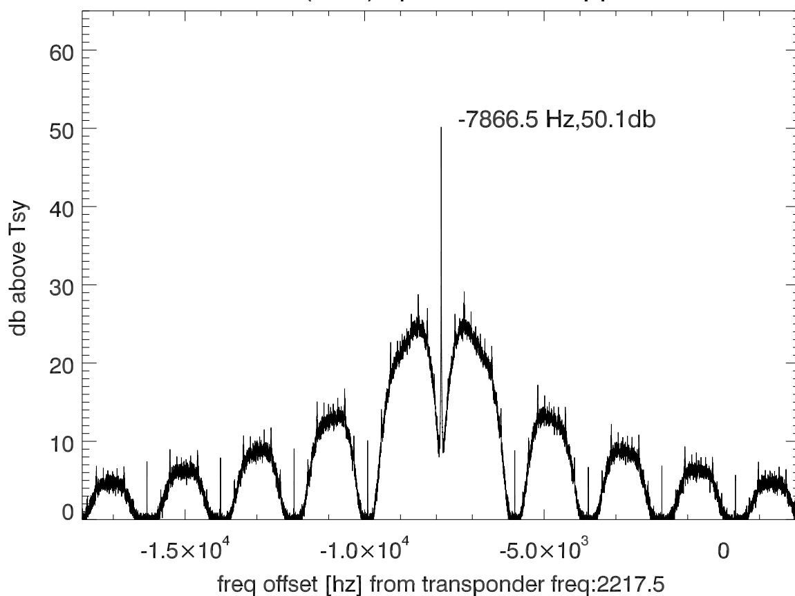
isee3 140624:200519 (UTC) spectra after doppler correction. PoIB
