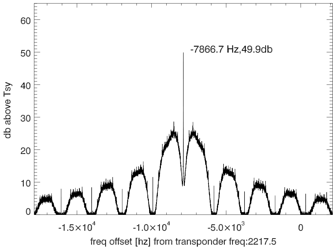
isee3 140624:200020 (UTC) spectra after doppler correction. PoIB
