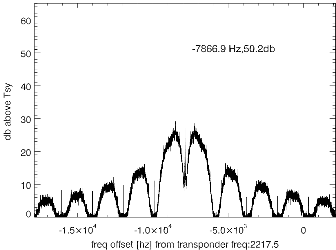
isee3 140624:195427 (UTC) spectra after doppler correction. PoIB
