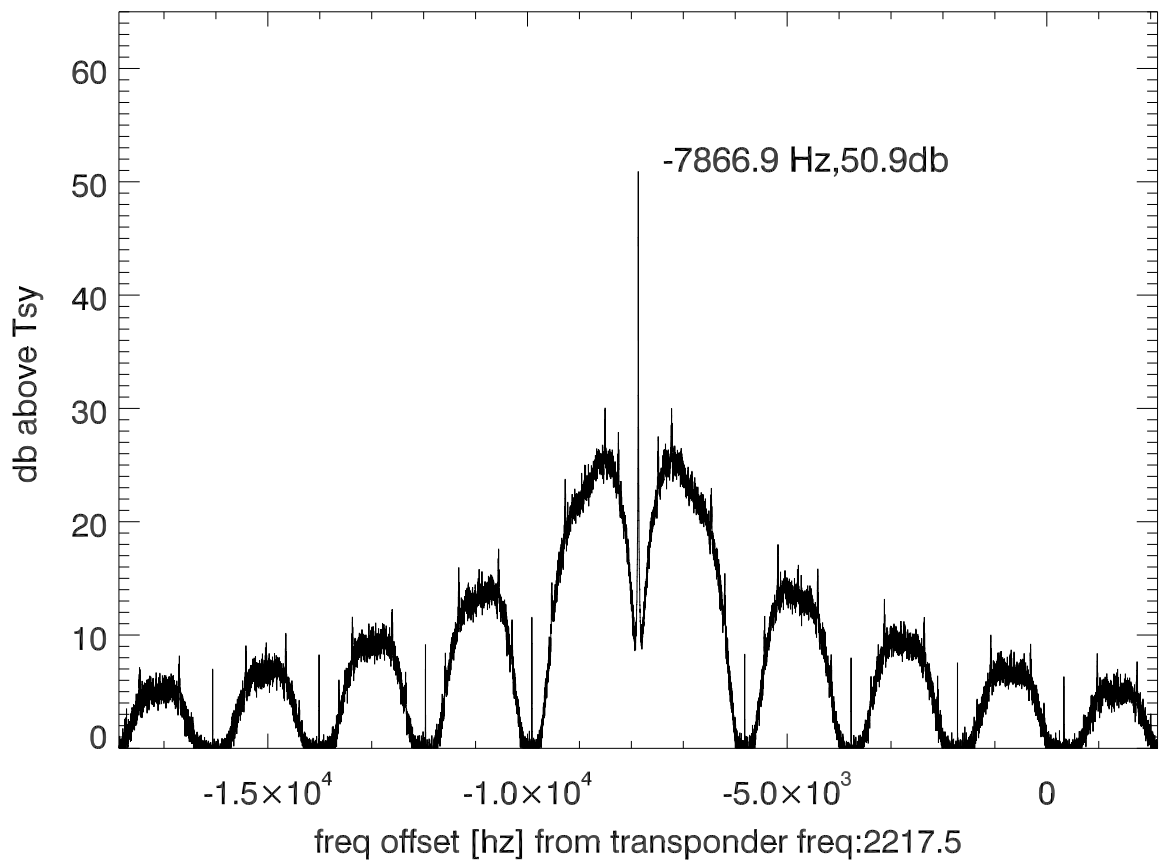
isee3 140624:194709 (UTC) spectra after doppler correction. PoIB
