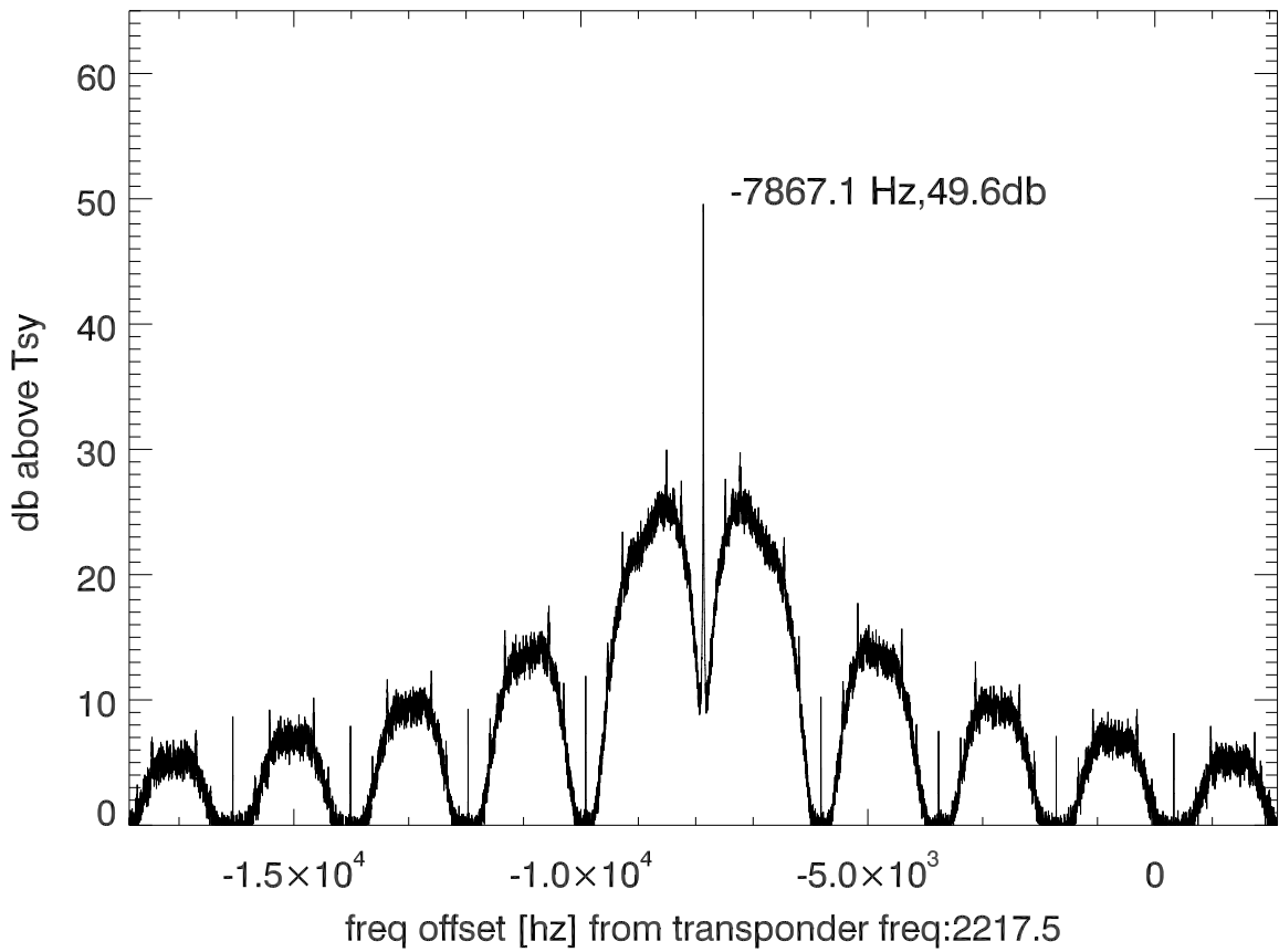
isee3 140624:194457 (UTC) spectra after doppler correction. PoIB
