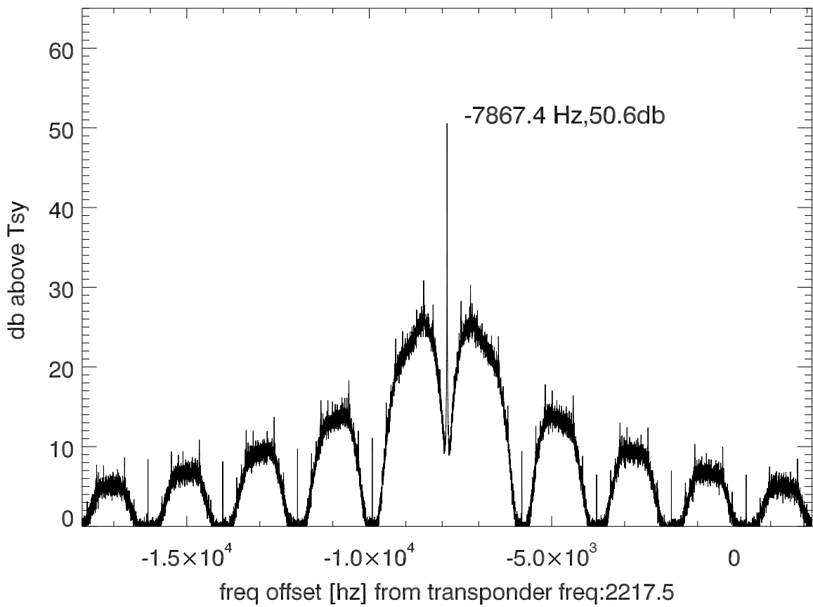
isee3 140624:193730 (UTC) spectra after doppler correction. PoIB
