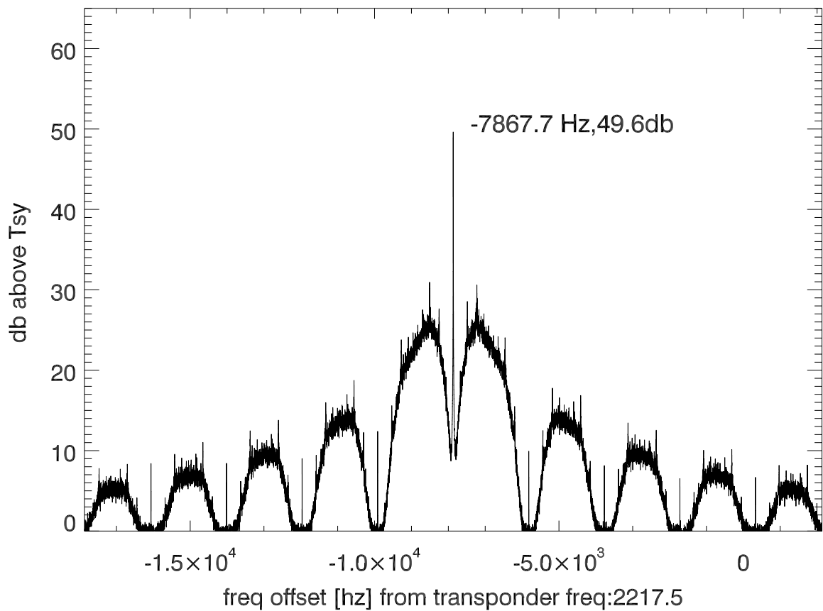
isee3 140624:192019 (UTC) spectra after doppler correction. PoIB
