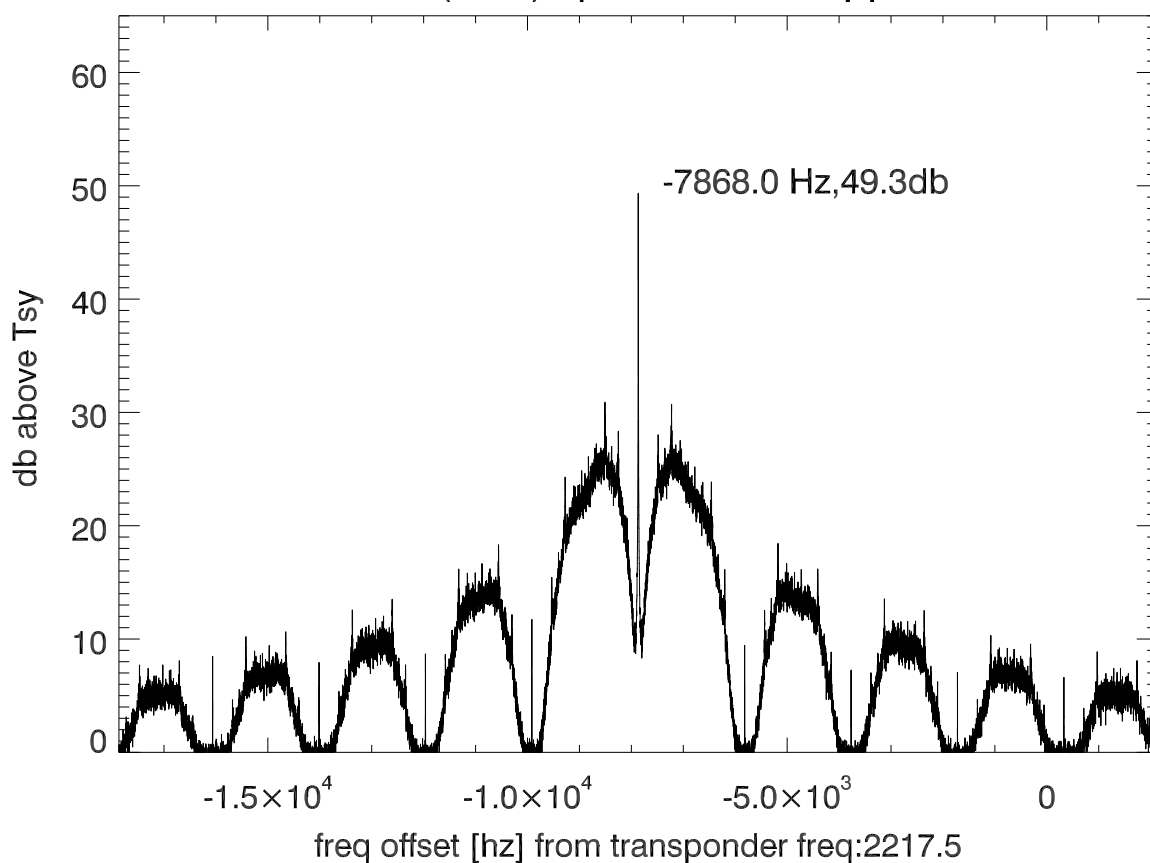
isee3 140624:190905 (UTC) spectra after doppler correction. PoIB
