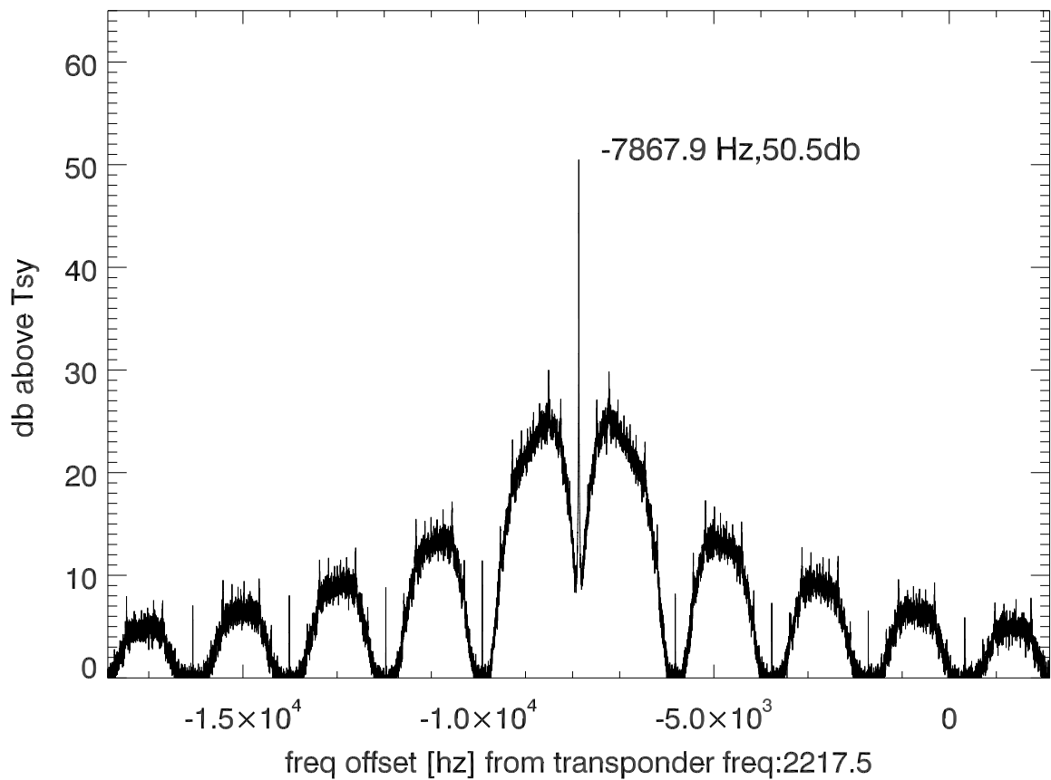
isee3 140624:190723 (UTC) spectra after doppler correction. PoIB
