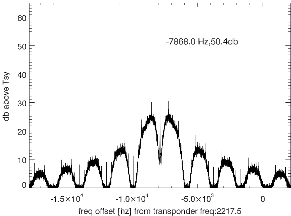
isee3 140624:190527 (UTC) spectra after doppler correction. PoIB
