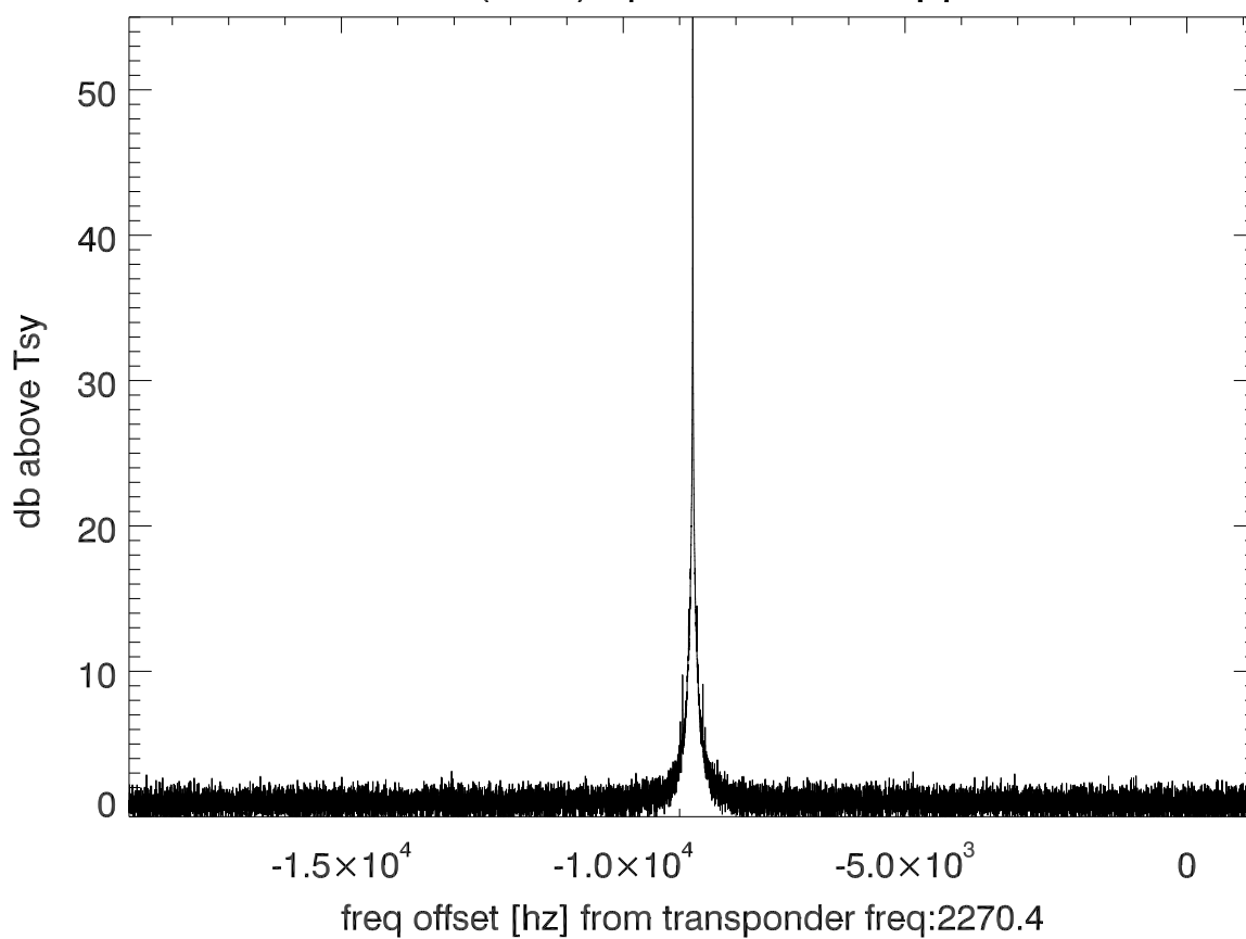
isee3 140620:194359 (UTC) spectra after doppler correction. PolB
