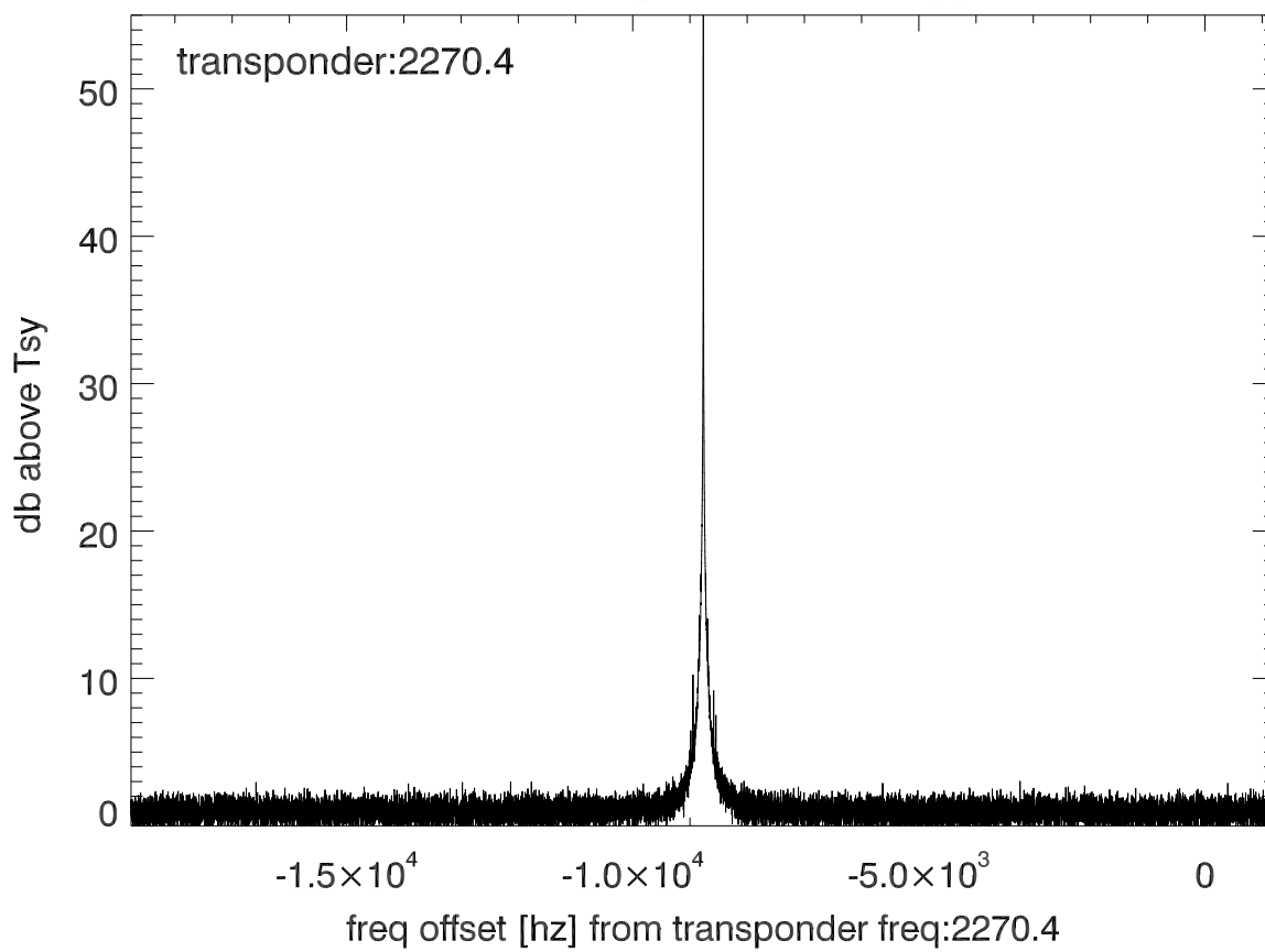
isee3 140620:194359 (UTC) spectra after doppler correction. PolA
