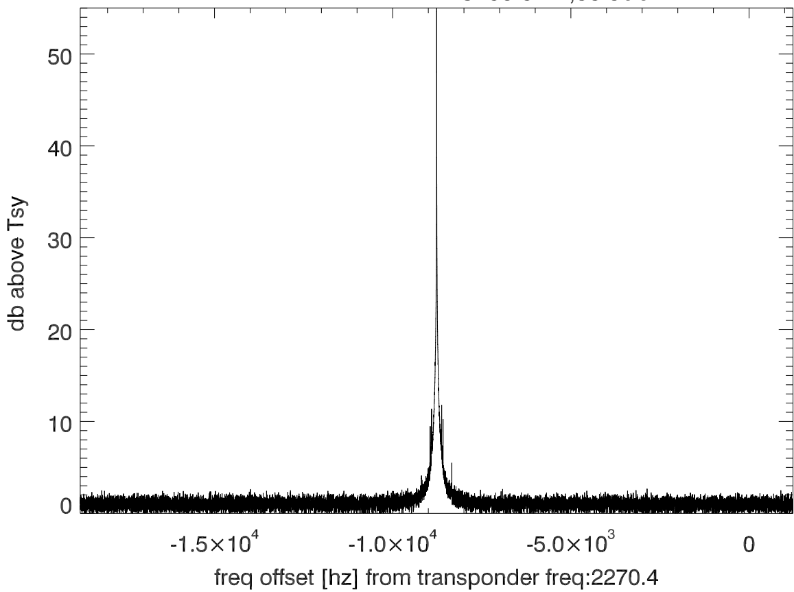
isee3 140620:193818 (UTC) spectra after doppler correction. PolB
