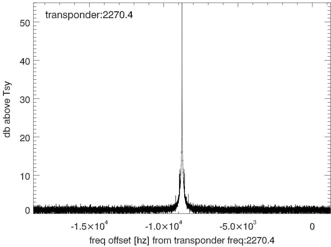
isee3 140620:193818 (UTC) spectra after doppler correction. PolA
