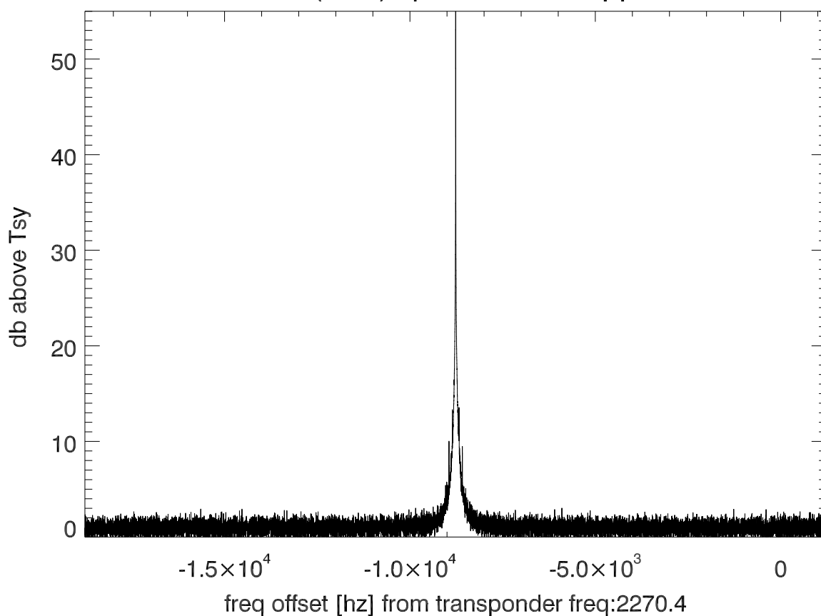
isee3 140620:192939 (UTC) spectra after doppler correction. PoIB
