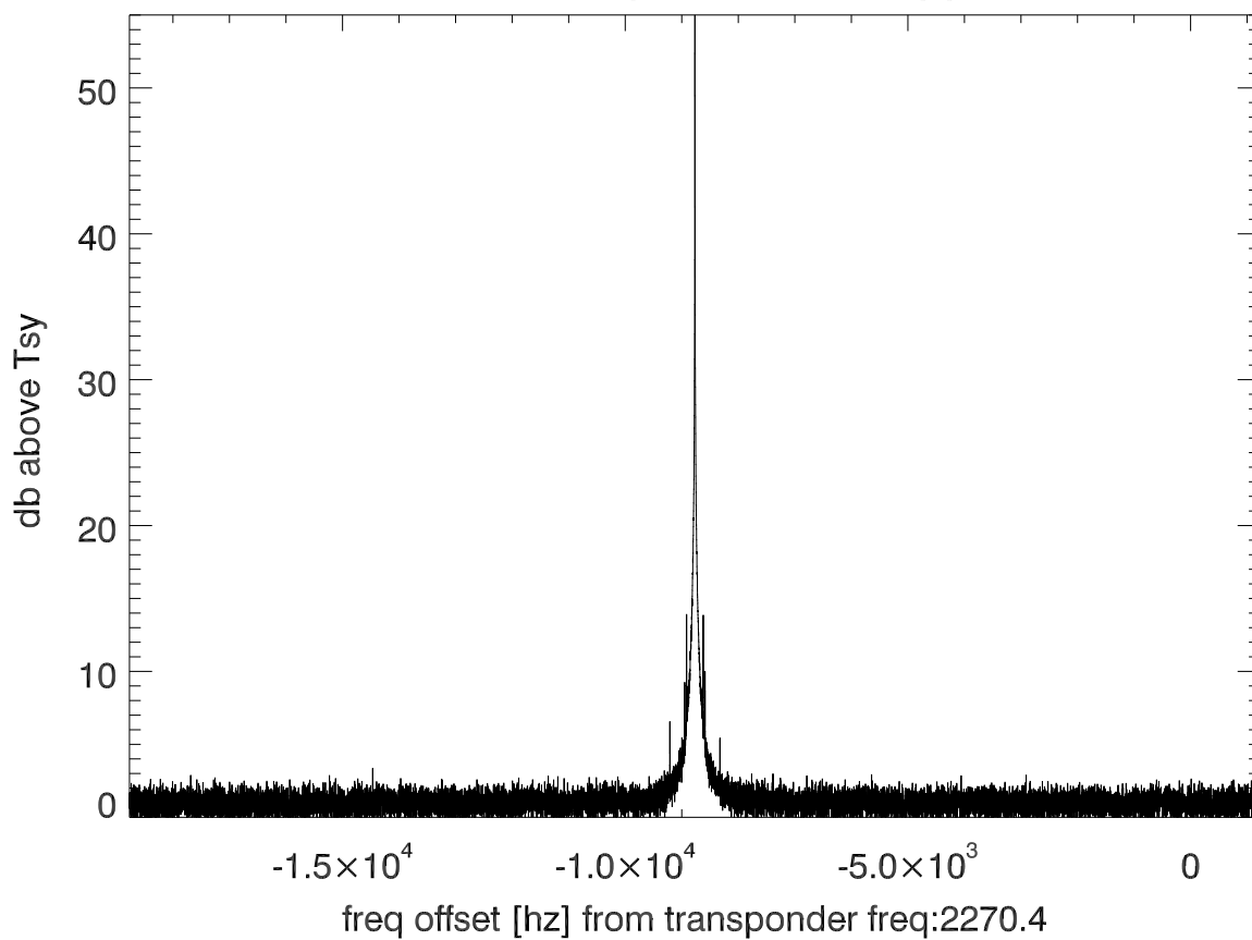
isee3 140620:192637 (UTC) spectra after doppler correction. PoIB
