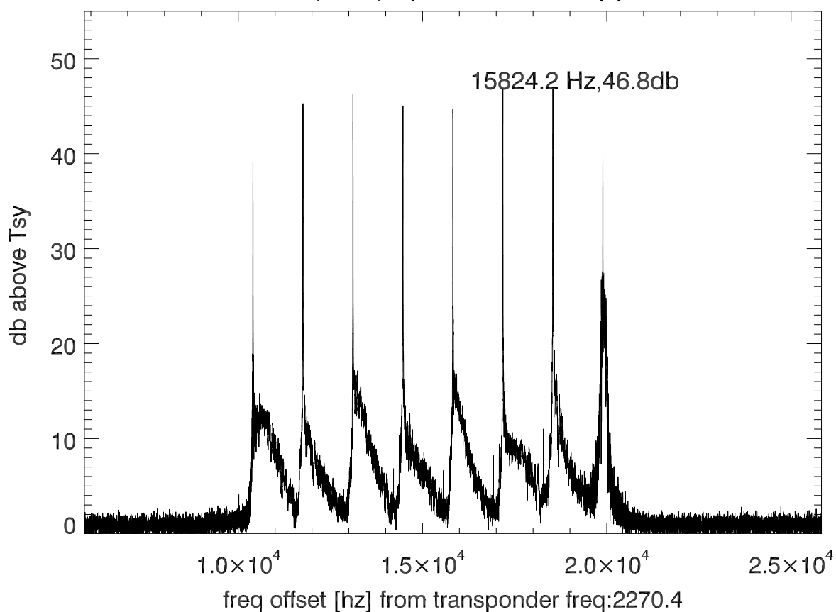
isee3 140620:192010 (UTC) spectra after doppler correction. PolB
