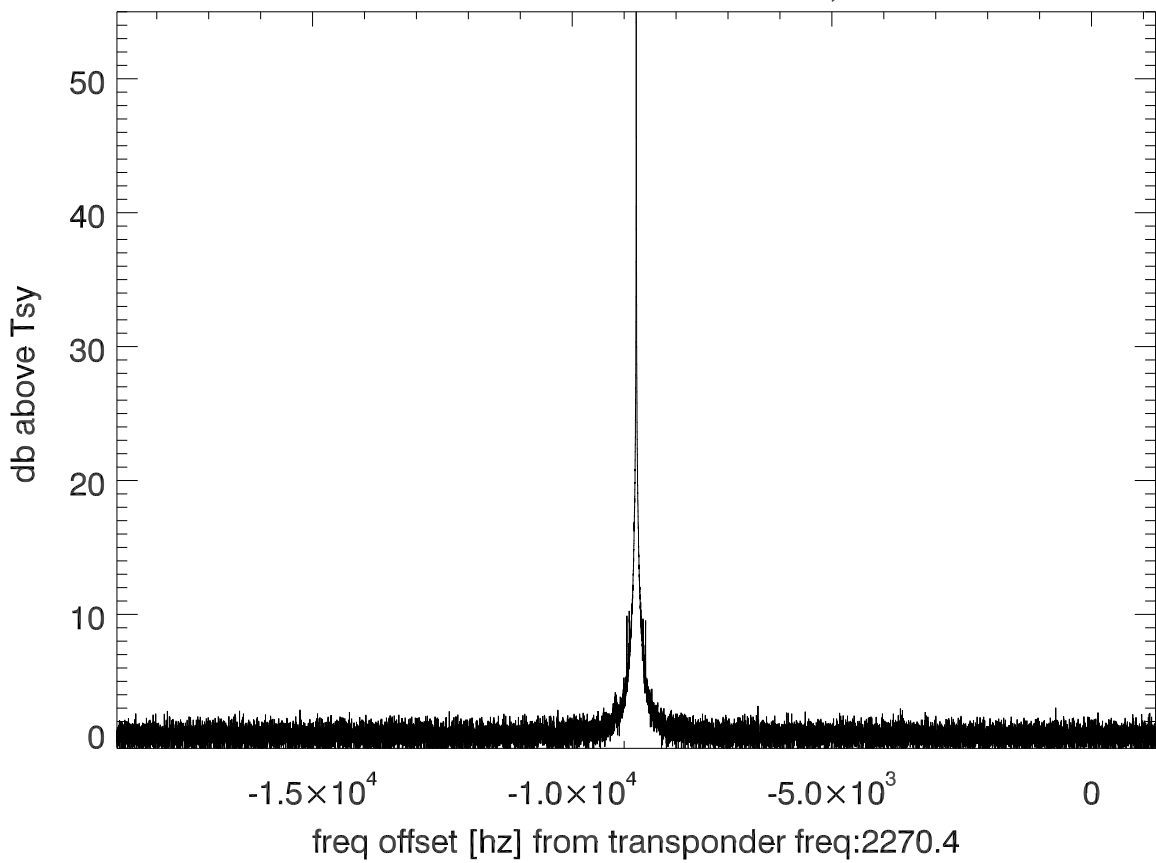
isee3 140620:191555 (UTC) spectra after doppler correction. PolB
