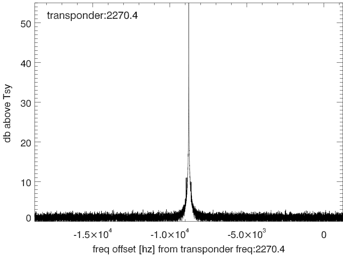
isee3 140620:191555 (UTC) spectra after doppler correction. PolA
