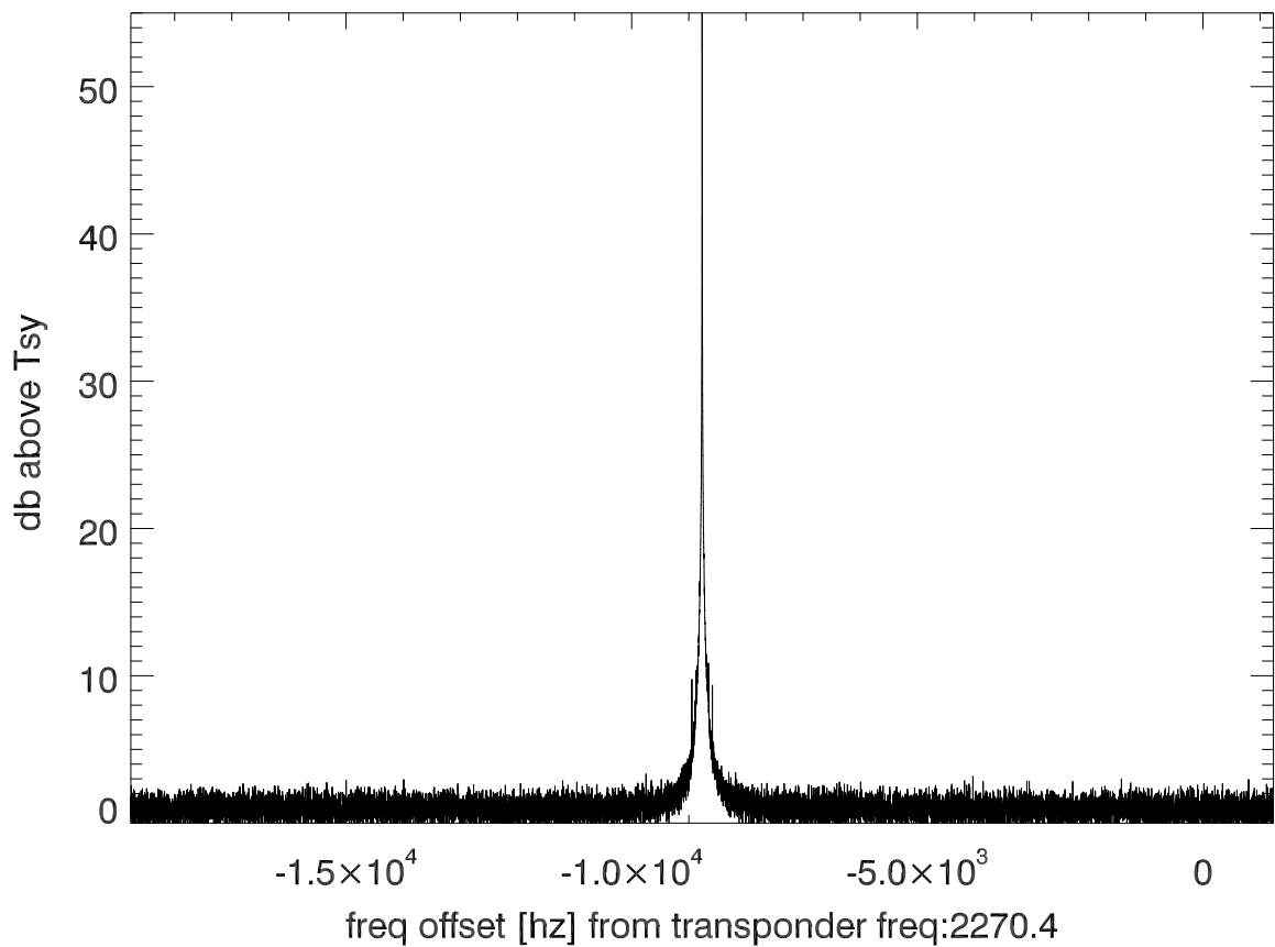
isee3 140620:191107 (UTC) spectra after doppler correction. PoIB
