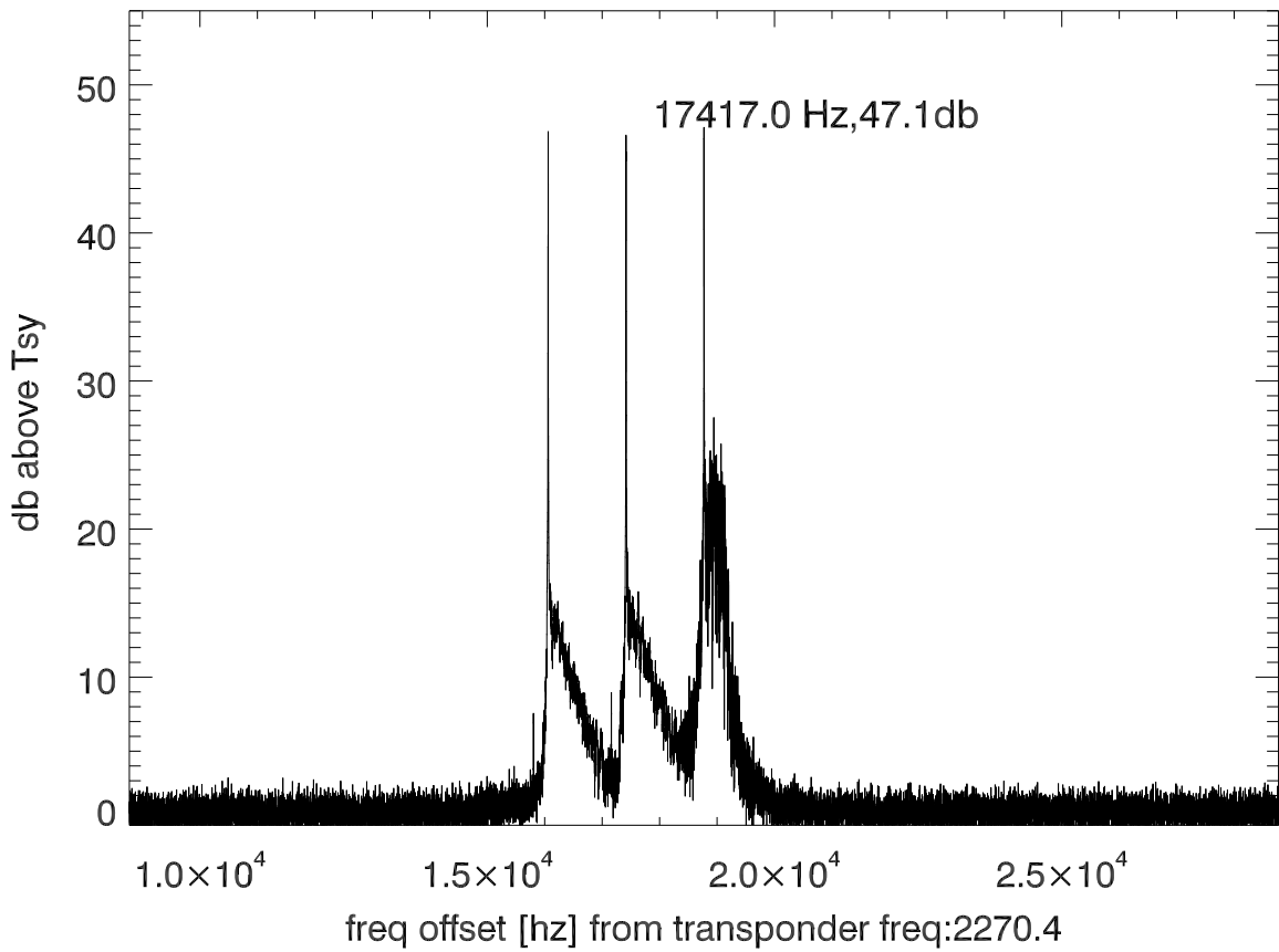
isee3 140620:190337 (UTC) spectra after doppler correction. PolB
