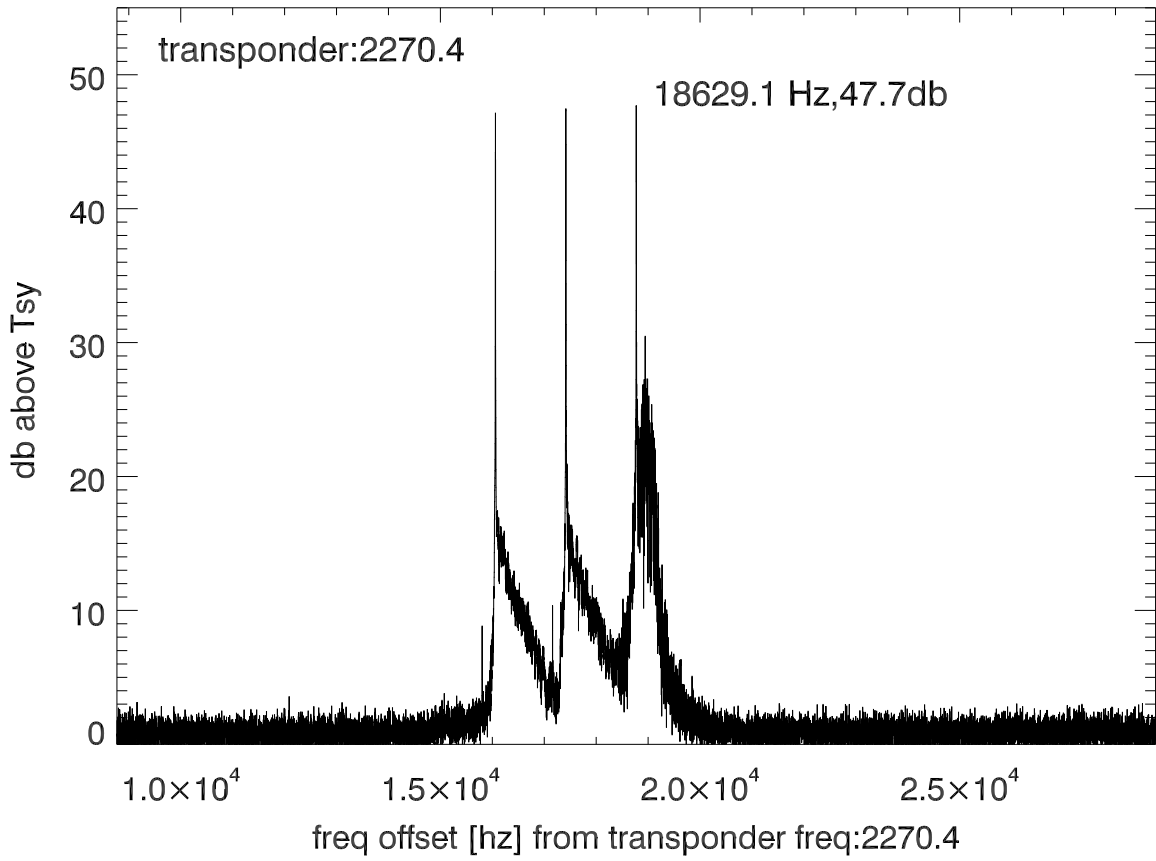
isee3 140620:190337 (UTC) spectra after doppler correction. PolA
